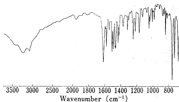
Fig. 2. IR Spectrum of II in KBr Disk
