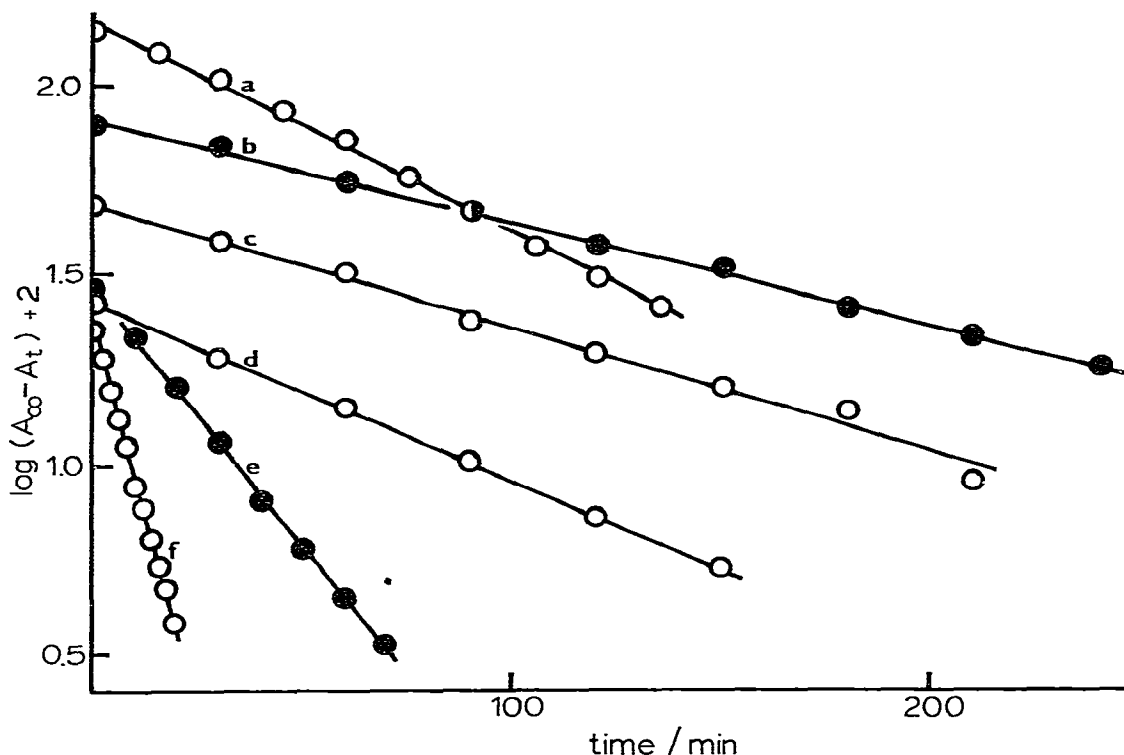
Fig. 1. Typical first order plots for the reactions of platinacyclobutanes (initial conc. \sim 2 \times 10^{-4} mol l ^{-1} ) with iodide and thiocyanate ions in CH 3 CN at 45.1°C. (a) [PtCl 2 (CH 2 CH 2 CH 2 CH 2 )(C 5 H 5 N) 2 ] + 20 Et 4 Ni; (b) [PtCl 2 (CH 2 CH 2 CH 2 CH 2 )(C 5 H 5 N) 2 ] + 40 KI + 0.6 C 5 H 5 N; (c) [PtCl 2 (CH 2 CMe 2 CH 2 CH 2 )(C 5 H 5 N) 2 ] + 20 Et 4 Ni (abs. \times 4 ); (d) [PtBr 2 (CH 2 CH 2 CH 2 CH 2 )(C 5 H 5 N) 2 ] + 20 Et 4 Ni; (e) [PtCl 2 (CH 2 CH 2 CH 2 CH 2 )(C 5 H 5 N) 2 ] + 20 KCNS; (f) [PtCl 2 (CH 2 CH 2 CH 2 CH 2 )(C 5 H 5 N) 2 ] + 40 Et 4 Ni + 197 Me 2 SO.
