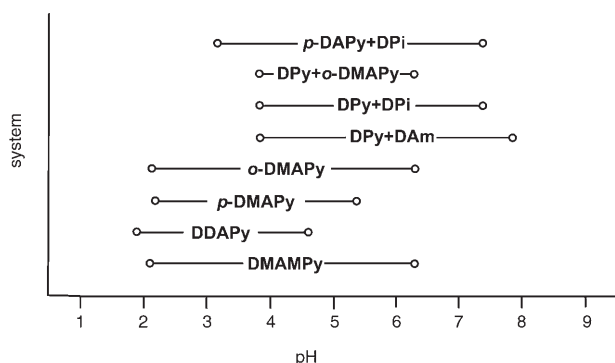
Figure 3. Horizontal segments represent the ideal half-height width of the I_f versus pH curves of each system. Their limiting values on the pH scale correspond to the pK_a values of base moieties responsible of the quenching processes.
