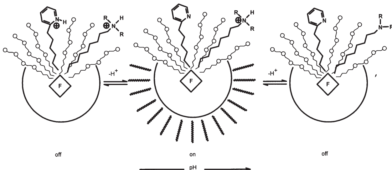
Scheme 3. Working scheme for the system based on the combination of one pyridine and one tertiary amine monobases ( F = pyrene, the pyridine-containing component is DPy , the tertiary-amine-containing component may be DAm or DPi ). Low pH passage from the “off” to the “on” form takes place at pH values crossing DPy pK_a . High pH passage from the “on” to the “off” form takes place at pH values crossing DAm or DPi pK_a .
