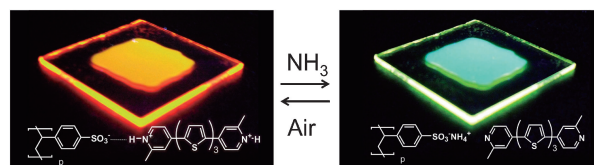
Figure 5. Photographs of the complex film containing 0.24 mol% 3Th-MP irradiated with 365-nm light under air (left) and ammonia (right). The inset of the photograph indicates plausible relevant structure.
