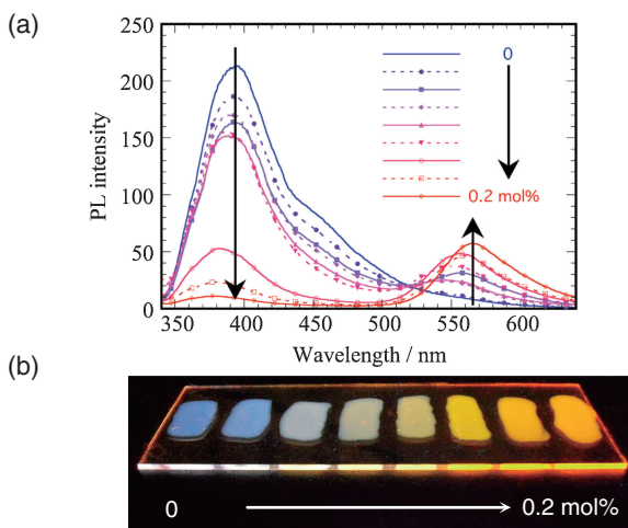
Figure 3. Change in PL spectra of aqueous solution (a) and photographs of 3Th-MP/PSS complex film (b) containing 3Th-MP at different ratio. The films in (b) were irradiated with 365-nm light.
