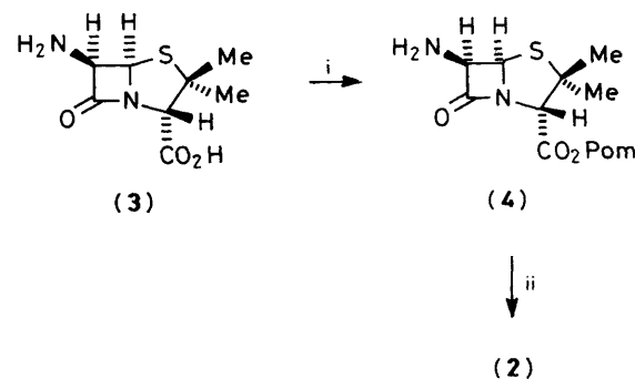
Scheme 2. Reagents: i, \text{ClCH}_2\text{OCOCMe}_3 , DBU; ii, \text{NBu}_4\text{NO}_2^- , \text{C}_5\text{H}_5\text{NH}^+(\text{HF})_x\text{F}^-
