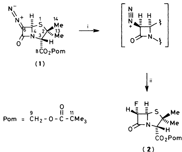
Scheme 1. Reagents: i, \text{C}_5\text{H}_5\text{NH}^+(\text{HF})_x\text{F}^- ; ii, \text{F}^-
