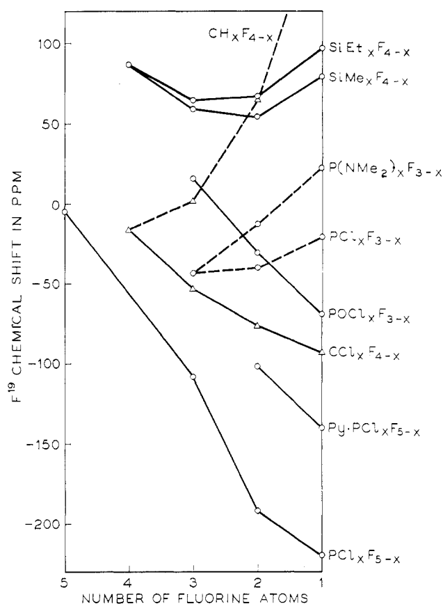
Fig. 2.— \text{F}^{19} chemical shift vs. number of fluorine atoms.
