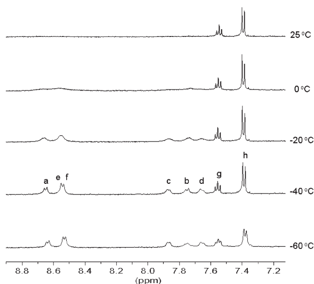
Figure 2. Variable-temperature 1 H NMR spectra of 2 in \text{CD}_2\text{Cl}_2 in aromatic region and assignment of aromatic protons. The resonance assignment referred to the structure shown in Figure 1.
