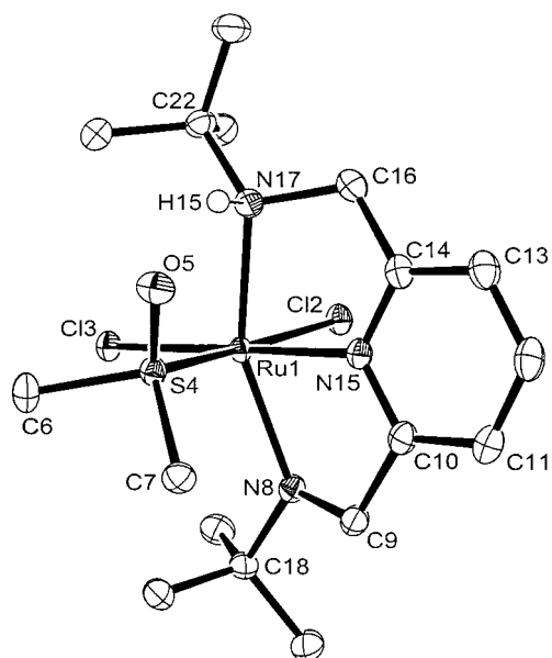
Figure 1. ORTEP drawing of \text{Ru}(\text{N}_2\text{py})\text{Cl}_2(\text{DMSO}) , showing intramolecular \text{NH}\cdots\text{O} hydrogen bonding.
