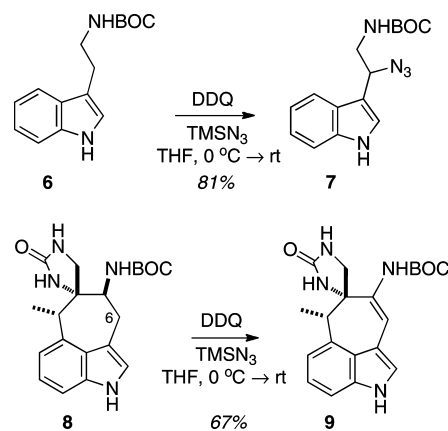
Scheme 2. Alternative C(6) Azide Introduction Attempt, Part 1
