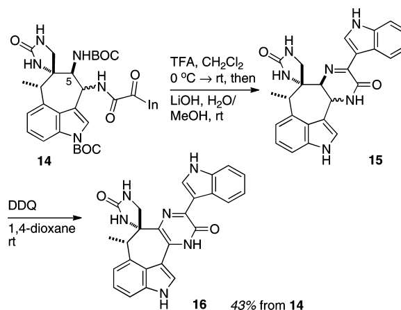
Scheme 5. Cyclocondensation to Form the Central Pyrazinone Ring
