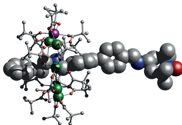
Figure 1. The structure of 1 in the crystal. The ring is shown as a ball-and-stick representation and the thread as a space-filling model. Color coding: Cr dark green, Ni purple, O red, C grey, N blue, F light green. H are not represented for clarity.
