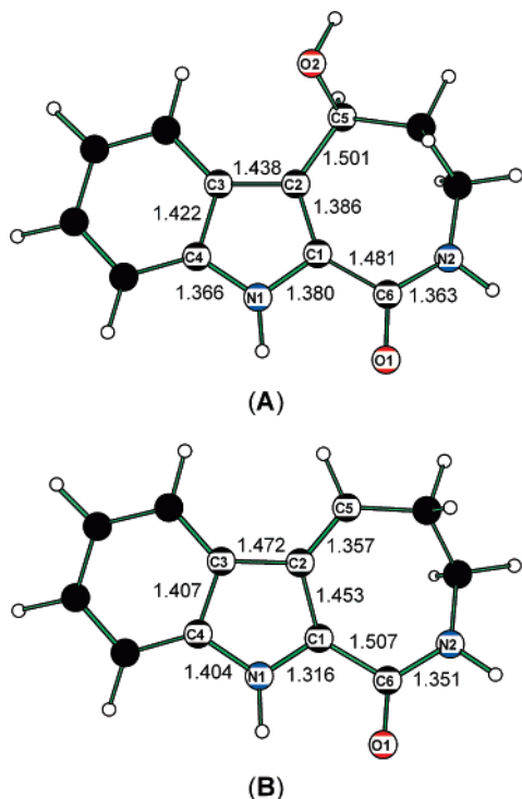
FIGURE 2. Calculated molecular structures of alcohol (±)-6 ( A ) and the cationic intermediate ( B ).
