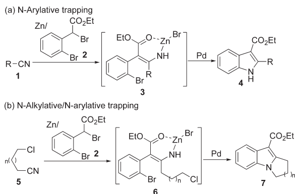
Scheme 1. Pd-Catalyzed Intramolecular Trapping Strategies for Tandem One-Pot Synthesis of (a) Indole and (b) N-Fused Indole Derivatives
