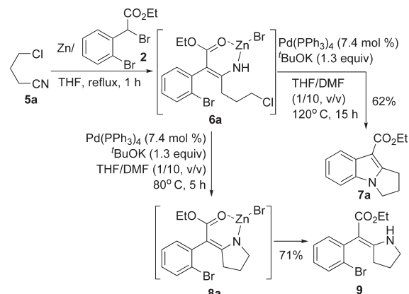
Scheme 2. Pd-Catalyzed N-Alkylative/N-Arylation Trapping of the Blaise Reaction Intermediate 6a
