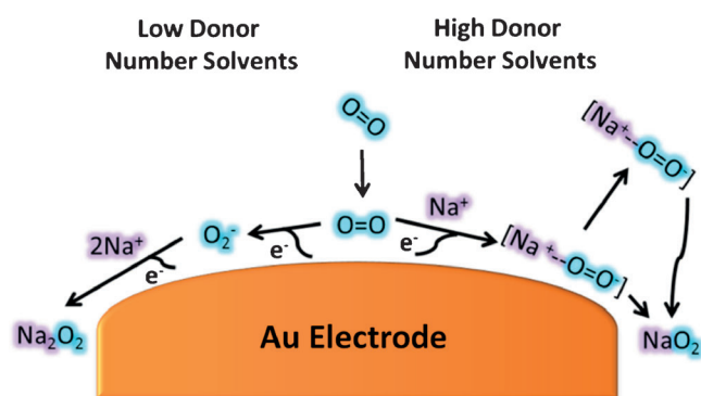
Scheme 1. Mechanism of oxygen reduction in non-aqueous solvents in the presence of Na + cations (with H 2 O ≤ 20 ppm).
