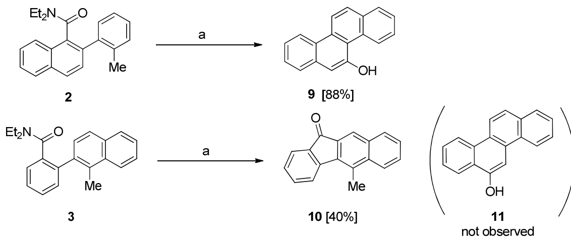
Scheme 1. Selectivities of the DreM-cyclization of ortho -aryl naphthamide 2 and benzamide 3 . Conditions: a) LDA (2.5 equiv), THF, r.t.
