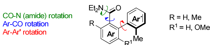
Figure 1. Potential rotational barriers of 2-amido-2'-methylbiaryls.
