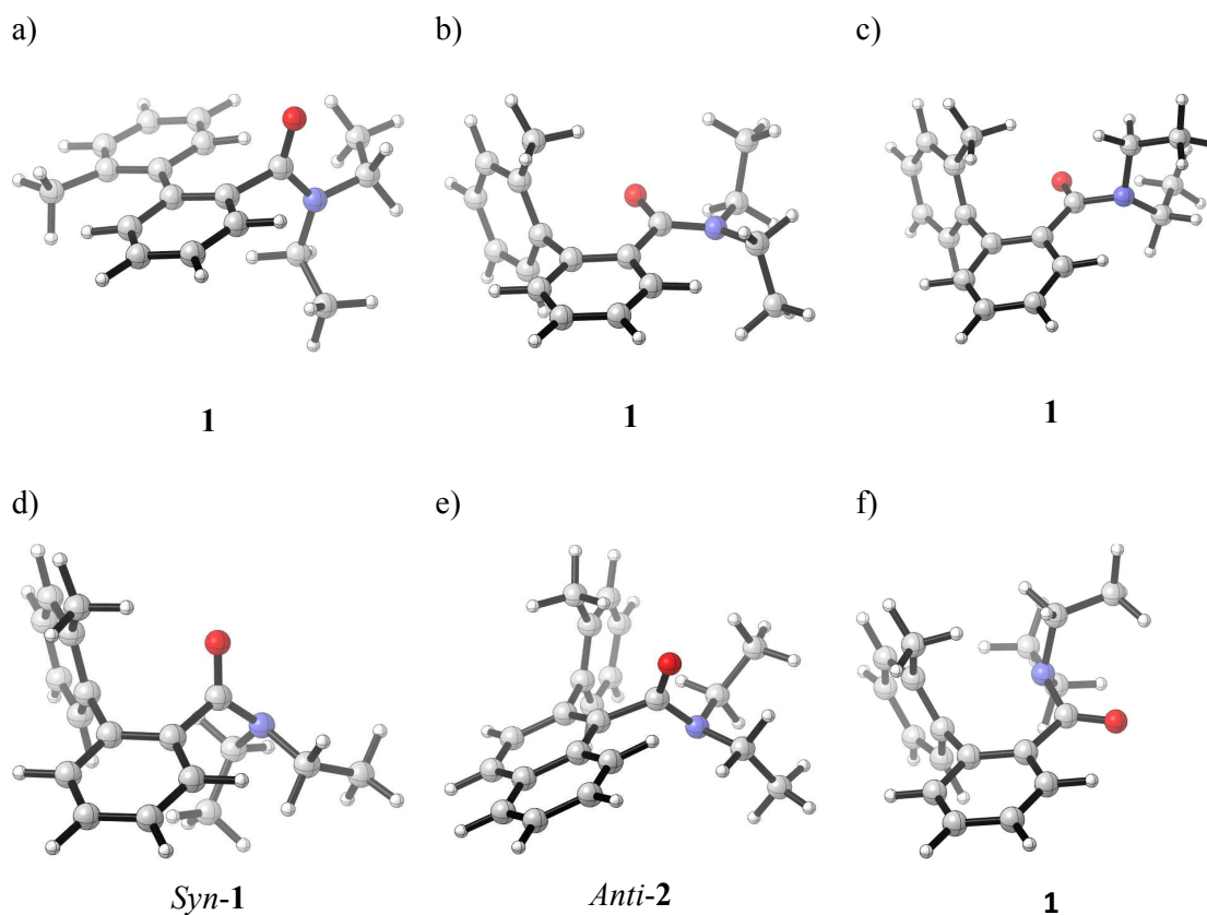
Figure 6. Calculated transition states for the different bond rotations of biaryl amides 1 and 2 .
