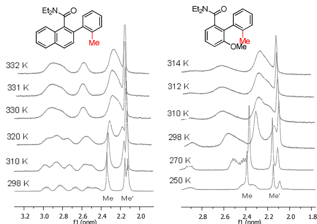
Figure 3. VT 1 H NMR of compounds 2 and 5 .
