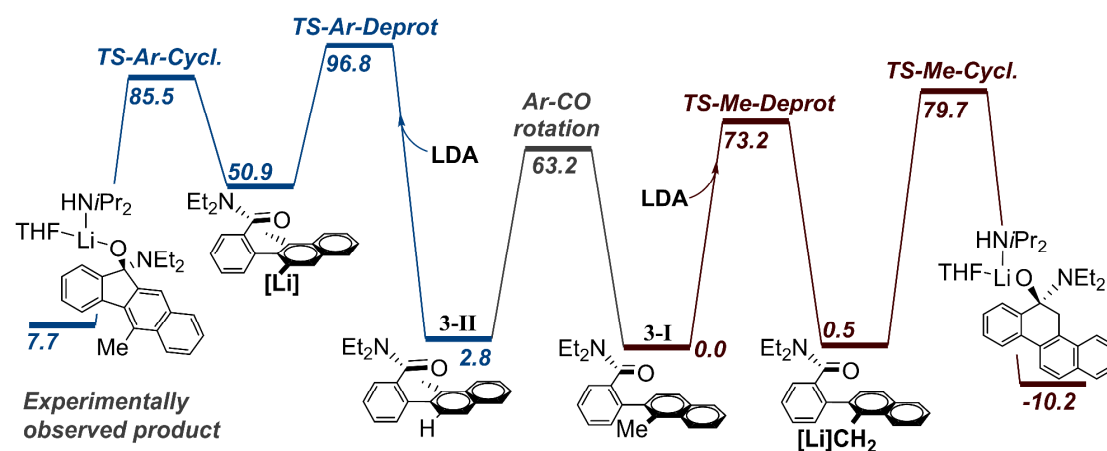
Figure 8: Comparison of the free energy (in kJ/mol) pathways of 2'-Me- and Ar' ring-deprotonation and the consecutive cyclization reactions of 2 (top) and 3 (bottom). Hydrogen atoms of the THF and i Pr 2 NH ligands and of the ethyl groups of the amide have been omitted for clarity. [Li] = -Li( i Pr 2 NH)(THF) 42
