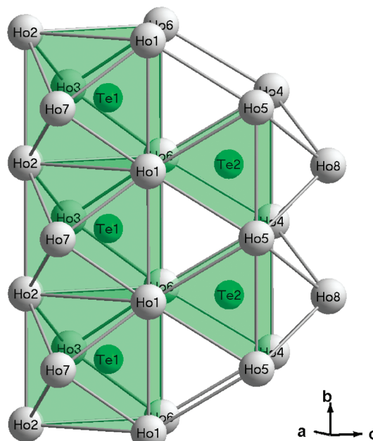
Figure 2. Section of an \sim[100] view of the Te1- and Te2-centered polyhedra in \text{Ho}_7\text{Au}_2\text{Te}_2 .
