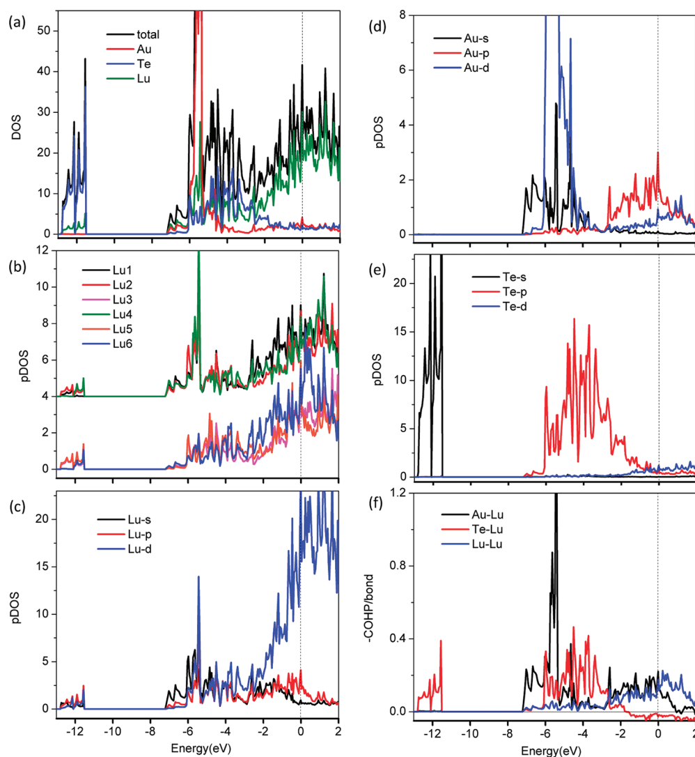
Figure 5. TB-LMTO-ASA electronic structure results for \text{Lu}_6\text{Au}_2\text{Te}_2 . (a) Total DOS and pDOS curves for Lu, Au, and Te. (b) DOS curves for separate Lu atoms. The data for Lu1, Lu2, and Lu4 are raised in order to distinguish them. (c and d) Orbital pDOS data for Lu, Au, and Te. (f) COHP (eV/bond-mol). The dashed lines mark the Fermi energy ( E_F ). (The comparable data for \text{Ho}_7\text{Au}_2\text{Te}_2 appear in Figure S2 in the Supporting Information.)
