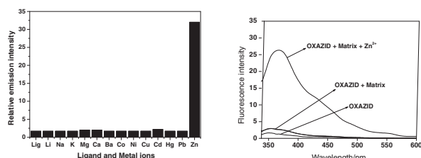
Figure 2. a) Relative emission intensity of oxazid ( 1 \times 10^{-6} M) with metal ions (100 equiv), b) competitive matrix experiment: emission spectra of oxazid alone (1 \mu g), oxazid + 5 \times 10^{-4} M each of \text{Li}^+ , \text{Na}^+ , \text{K}^+ , \text{Mg}^{2+} , \text{Ca}^{2+} , \text{Ba}^{2+} , \text{Co}^{2+} , \text{Ni}^{2+} , \text{Cu}^{2+} , \text{Cd}^{2+} , \text{Pb}^{2+} , and \text{Hg}^{2+} and oxazid + matrix + \text{Zn}^{2+} ( 10^{-4} M).
