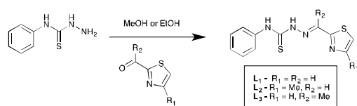
Scheme 1 General synthesis of \text{L}_1 - \text{L}_3
