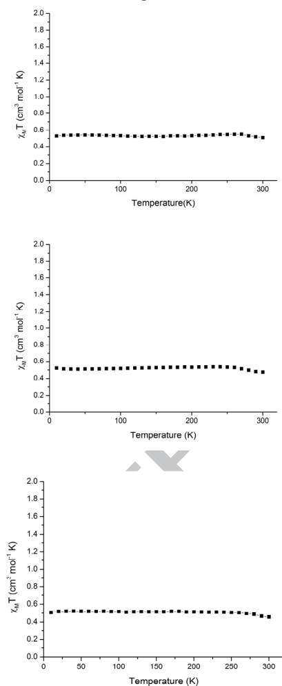
Fig 7 Plots of \chi_{\text{MT}} vs. T for [\text{Fe}(\text{L}_1)_2](\text{NO}_3) \cdot \text{H}_2\text{O} (top), [\text{Fe}(\text{L}_2)_2](\text{NO}_3) \cdot \text{H}_2\text{O} (middle) and [\text{Fe}(\text{L}_3)_2](\text{NO}_3) \cdot \frac{3}{4}\text{H}_2\text{O} (bottom).
