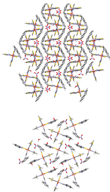
Fig. 5 Packing diagrams of [\text{Fe}(\text{L}_1)_2](\text{NO}_3)\cdot\text{H}_2\text{O} (top) showing spiralled layer formation and [\text{Fe}(\text{L}_2)_2](\text{NO}_3)\cdot\text{H}_2\text{O} showing both the orientation of the packing along the crystallographic c -axis (bottom).
