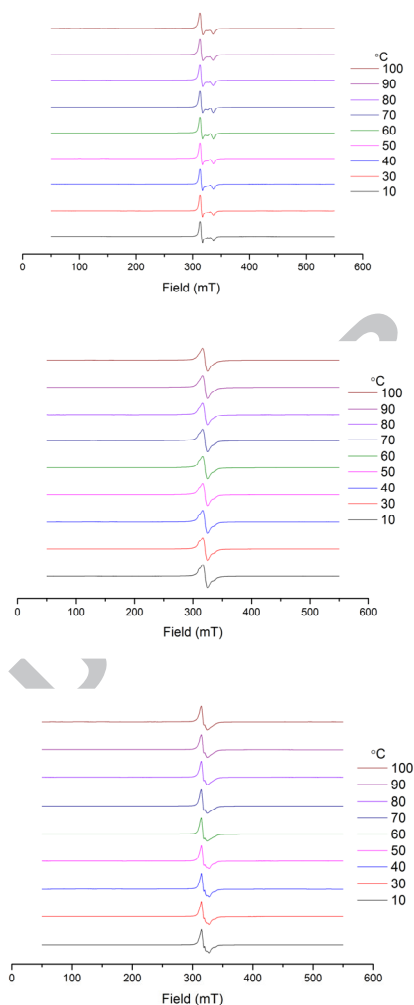
Fig. 6 Variable temperature EPR of [\text{Fe}(\text{L}_1)_2](\text{NO}_3)\cdot\text{H}_2\text{O} (top), [\text{Fe}(\text{L}_2)_2](\text{NO}_3)\cdot\text{H}_2\text{O} (middle) and [\text{Fe}(\text{L}_3)_2](\text{NO}_3)\cdot\frac{3}{4}\text{H}_2\text{O} (bottom).
