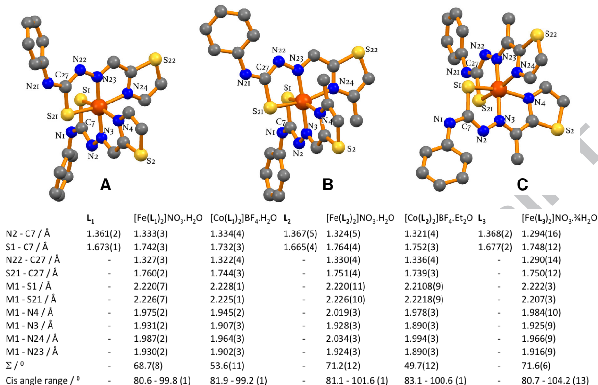
Fig. 4 Molecular structures (top) of [Fe(L 1 ) 2 ](NO 3 )·H 2 O (A), [Fe(L 2 ) 2 ](NO 3 )·H 2 O (B), and [Fe(L 3 ) 2 ](NO 3 )·3/4H 2 O (C) showing numbering scheme. Nitrate counter anion, interstitial water molecules and hydrogen atoms are omitted for clarity – see ESI for additional figures of the molecular structures. Table of selected bond lengths and angles (bottom) for all structurally characterised ligands and complexes. Σ values for complexes are also tabulated for structurally characterised Fe(III) and Co(III) complexes.
