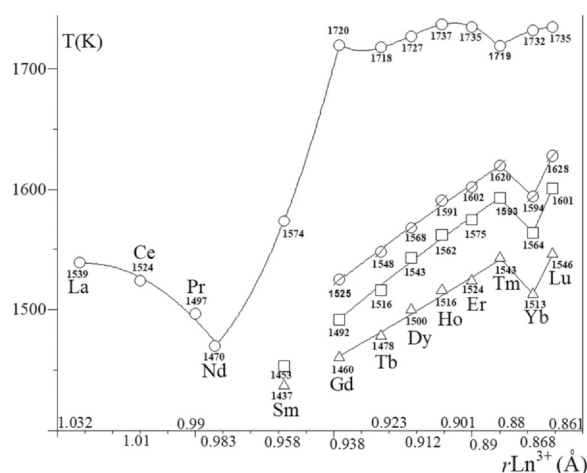
Fig. 2. Phase-transition temperatures of \text{EuLnCuS}_3 ( \text{Ln} = \text{La-Nd} [98], \text{Gd} [99], \text{Dy} [58], \text{Ho} [57], for the \text{Sm} , \text{Tb} , \text{Tm} , \text{Yb} and \text{Lu} compounds the phase transition temperatures were measured in this work): \Delta \alpha - \beta ; \square \beta - \gamma ; and \circ \gamma - \beta polymorphic transitions and \bigcirc incongruent melting.
