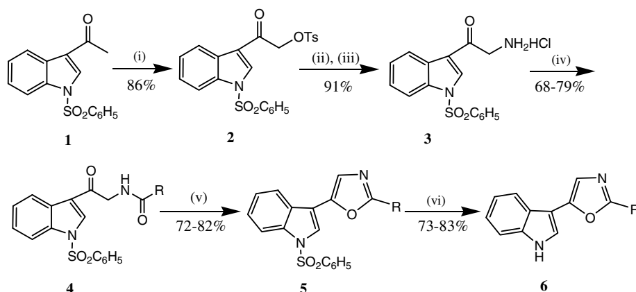
Scheme 1. Synthesis of 5-(3-indolyl)oxazoles. Reagents and conditions: (i) \text{C}_6\text{H}_5\text{I}(\text{OH})\text{OTs} , \text{CH}_3\text{CN} , rt; (ii) HMTA, \text{CHCl}_3 ; (iii) \text{HCl} , reflux; (iv) \text{RCOCl} , \text{Et}_3\text{N} , 0-5^\circ\text{C} ; (v) PTSA, \text{EtOH} , reflux; (vi) \text{NaOH} , \text{EtOH}-\text{H}_2\text{O} , reflux.
