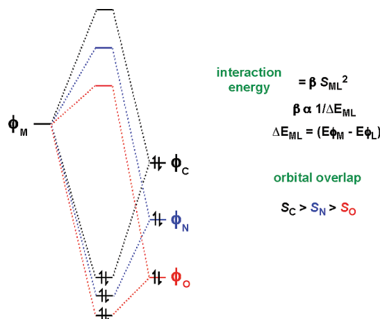
Figure 1. Angular overlap arguments show that both the interaction energy and orbital overlap favor C-based over N- and O-based ligands in terms of field strength.
