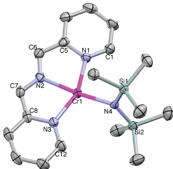
Figure 5. Molecular view of (\text{smif})\text{CrN}(\text{TMS})_2 ( 4-Cr ). Selected bond distances (Å) and angles (deg): \text{Cr1N1} , 2.0887(14) ; \text{Cr1N2} , 2.0416(14) ; \text{Cr1N3} , 2.0864(15) ; \text{Cr1N4} , 2.0260(12) ; \text{N2C6} , 1.332(2) ; \text{N2C7} , 1.320(2) ; \text{N4Si1} , 1.6967(14) ; \text{N4Si2} , 1.6913(14) ; \text{N1Cr1N3} , 157.07(6) ; \text{N2Cr1N4} , 168.76(6) ; \text{N1Cr1N2} , 78.80(6) ; \text{N1Cr1N4} , 101.04(6) ; \text{N2Cr1N3} , 78.35(6) ; \text{N3Cr1N4} , 101.74(6) ; \text{Cr1N1C1} , 129.05(12) ; \text{Cr1N1C5} , 112.12(12) ; \text{Cr1N3C12} , 129.57(13) ; \text{Cr1N3C8} , 113.02(12) ; \text{Cr1N2C6} , 115.65(13) ; \text{Cr1N2C7} , 115.77(13) ; \text{C6N2C7} , 128.48(17) ; \text{Cr1N4Si1} , 110.97(7) ; \text{Cr1N4Si2} , 122.23(7) .
