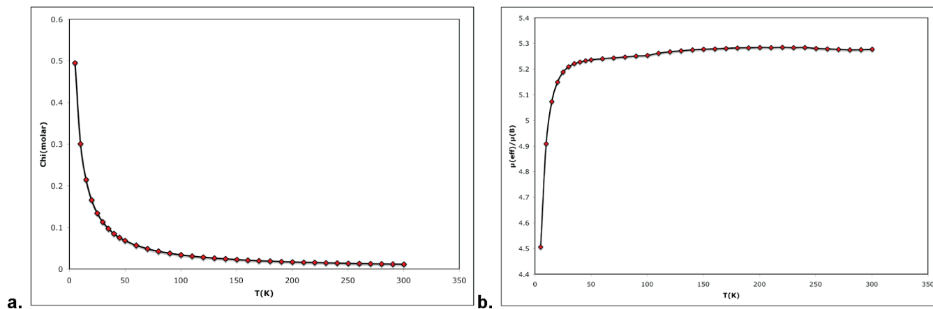
Figure 4. a. Molar Susceptibility ( \chi_M ) of (Arpy 2 N)FeBr ( 2-Fe ) as a function of T (K). b. Magnetic moment ( \mu_{\text{eff}} in \mu_B ) of 2-Fe as a function of T (K).
