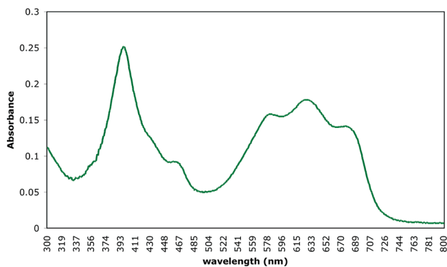
Figure 6. UV-vis spectrum of (\text{smif})\text{CrN}(\text{TMS})_2 ( 4-Cr ): 396\text{ nm} ( \epsilon \sim 27\,000\text{ M}^{-1}\text{cm}^{-1} ), 424\text{ nm} (sh, \epsilon \sim 12\,500\text{ M}^{-1}\text{cm}^{-1} ), 461\text{ nm} ( \epsilon \sim 9\,500\text{ M}^{-1}\text{cm}^{-1} ), 581\text{ nm} ( \epsilon \sim 17\,000\text{ M}^{-1}\text{cm}^{-1} ), 627\text{ nm} ( \epsilon \sim 19\,000\text{ M}^{-1}\text{cm}^{-1} ), 675\text{ nm} ( \epsilon \sim 15\,000\text{ M}^{-1}\text{cm}^{-1} ).
