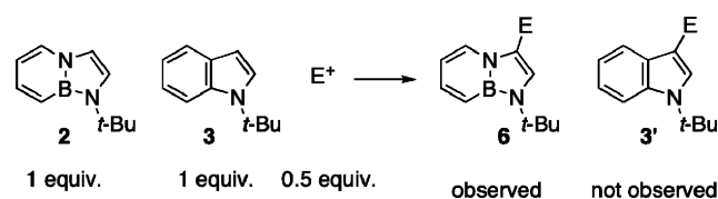
Scheme 4. EAS Competition Experiment with Dimethyliminium Chloride As the Electrophile
