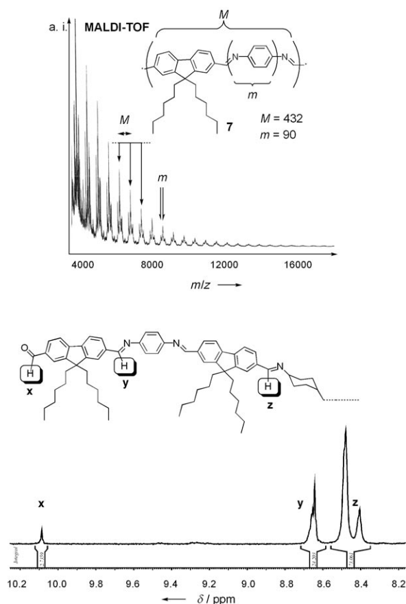
Figure 2. Top: MALDI-TOF spectroscopy in a ditanol matrix of compound 7 bearing repetitive monomeric units (with their corresponding mass fragments M and m ) up to a degree of polymerization (DP) of 34 (MW ≈ 15000). Bottom: 1 H NMR spectrum of a mixed polymeric structure incorporating both 1,4-phenylenediamine and trans -1,4-cyclohexanediamine (1:1) in chloroform ( c = 10 −4 M) at RT with labeled characteristic signals of: remaining aldehyde ( x ), aromatic imine ( y ), and ( cis + trans ) aliphatic imine ( z ).
