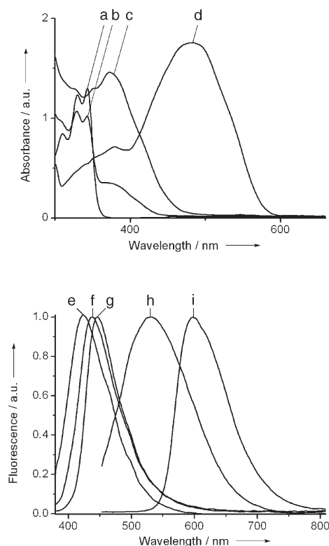
Figure 5. Top: UV-visible absorption spectra of CDL I in chloroform for various concentrations in \text{CF}_3\text{CO}_2\text{D} (a: reference 2 ; b: CDL I , 0 M; c: CDL I , 10^{-1} \text{ M} ; d: CDL I , 1 M). Bottom: Normalized fluorescence spectra of CDL I in chloroform for various concentrations in \text{CF}_3\text{CO}_2\text{D} (e: reference 2 ; f: CDL I , 0 M; g: CDL I , 10^{-1} \text{ M} ; h: CDL I , 10^{-1} \text{ M} ; i: CDL I , 1 M). For both experiments, the proton concentration values are given for a solution of initial concentration 5.12 \times 10^{-2} \text{ M} in dialdehyde A ; the spectra were recorded after equilibration and subsequent dilution to reach the values of [\text{A}] = 2.6 \times 10^{-5} \text{ M} (top) and [\text{A}] = 2.6 \times 10^{-6} \text{ M} (bottom). Dilution is not expected to change the equilibria; as the measurements are conducted in chloroform, the protonation state should not be significantly affected; furthermore, no change in spectra over time has been observed.
