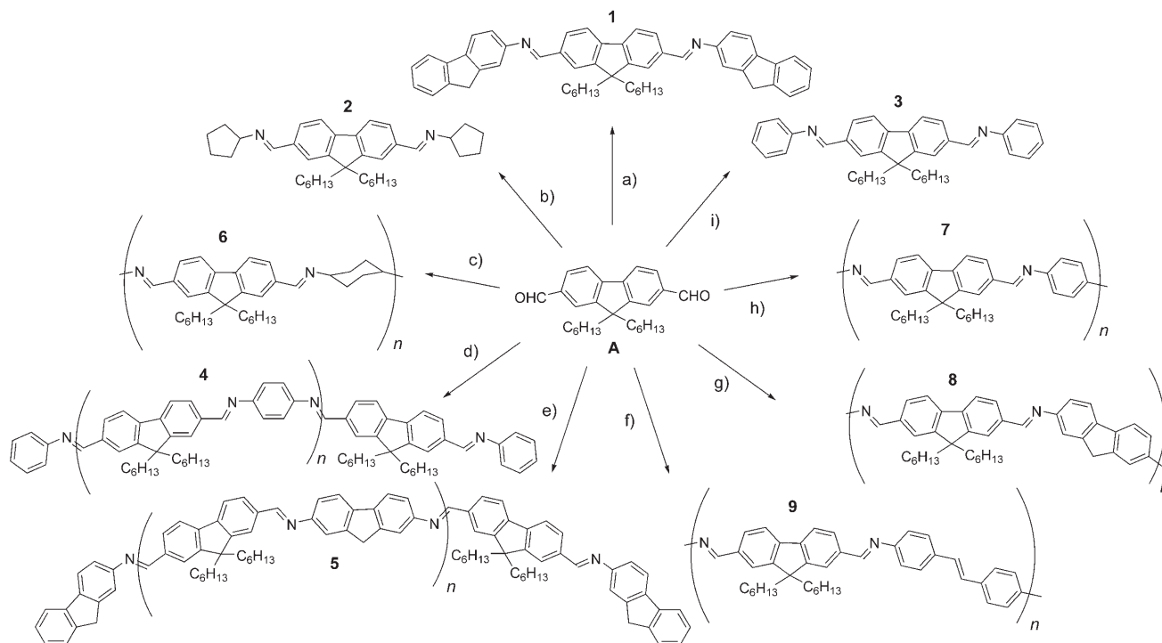
Scheme 2. Synthetic scheme for the syntheses of oligomeric and polymeric structures 1–9 from 2,7-fluorenebisoxaldehyde A . All the reactions were set up by mixing A with imine derivatives in ethanol for 12 h. a) 2 equiv aminofluorene. b) 3 equiv cyclopentylamine. c) 1 equiv trans -1,4-cyclohexyldiamine. d) 0.5 equiv 1,4-phenylenediamine, 1 equiv aniline. e) 0.5 equiv 2,7-diaminofluorene, 1 equiv 2-aminofluorene. f) 1 equiv 4,4'-diaminostilbene. g) 1 equiv 2,7-diaminofluorene. h) 1 equiv 1,4-phenylenediamine.
