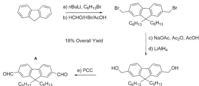
Scheme 1. Synthetic scheme for the five steps sequence leading to 2,7-fluorenebisoxaldehyde A from fluorene. a) n BuLi (2 equiv), slow addition (0.5 h), THF, -78^{\circ}\text{C} ; then 1-bromohexane, 3 equiv, -78^{\circ}\text{C} \rightarrow \text{RT} , 12 h, quantitative yield. [26] b) Paraformaldehyde (10 equiv), 0^{\circ}\text{C} ; then 30% solution of HBr in acetic acid, 65^{\circ}\text{C} , 24 h, 88%. [26] c) Anhydrous sodium acetate (10 equiv), acetic acid anhydride (10 equiv), acetic acid, reflux, 24 h, mixture of mono and bisacetate (2:1), 30%. d) \text{LiAlH}_4 (10 equiv), THF, reflux 18 h, 92%. e) PCC (20 equiv), molecular sieves (50 mass %), silica gel (50 mass %), \text{CH}_2\text{Cl}_2 , 4 h, then RT, 12 h, 75%.
