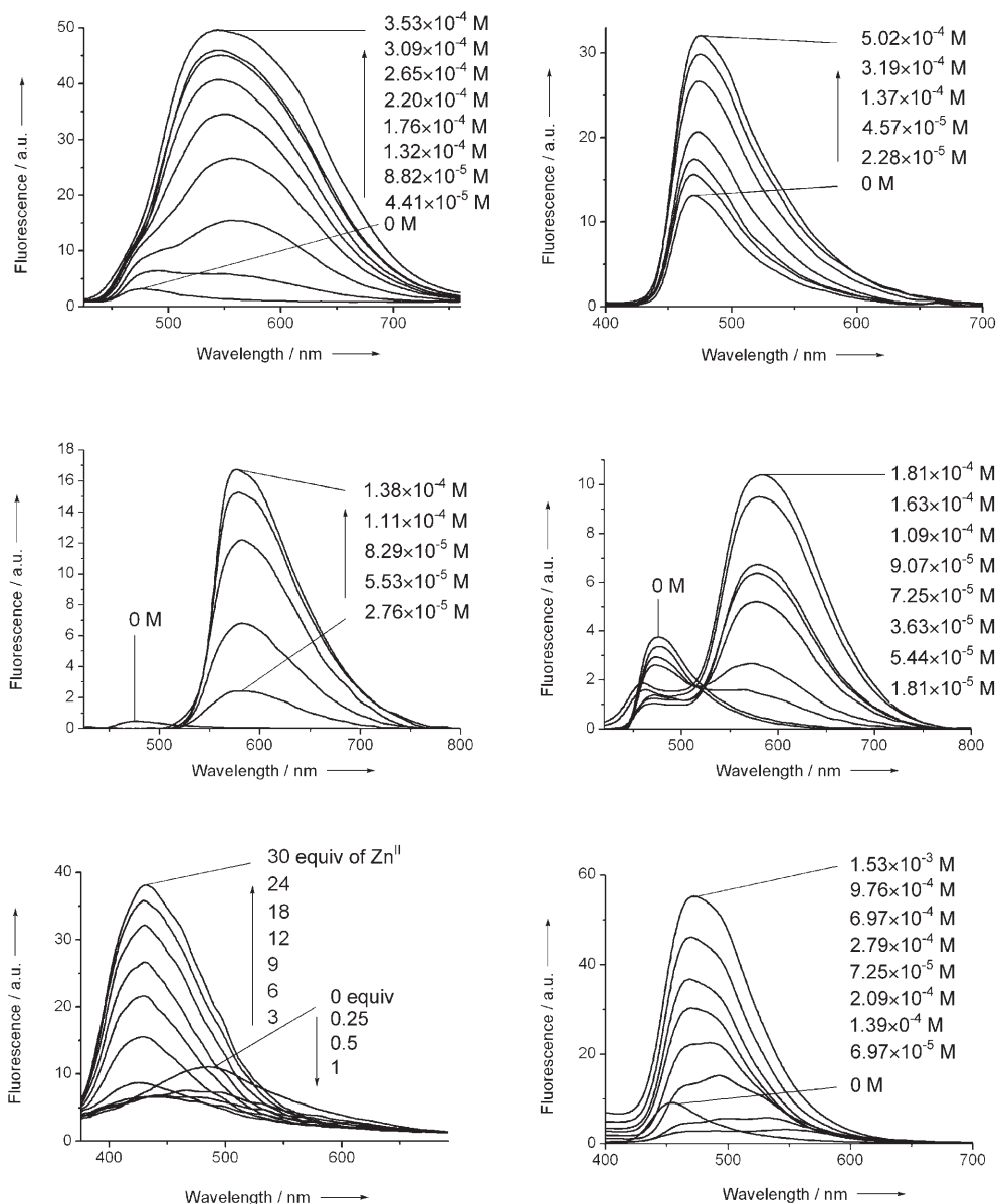
Figure 7. Top left: Fluorescence spectra at 298 K in \text{CHCl}_3 of compound 7 ( c = 4 \times 10^{-6} M) when adding increasing amounts of \text{Ag}(\text{OTf}) solubilized in \text{MeNO}_2 . Excitation wavelength 390 nm for all the series. Top right: Fluorescence spectra at 298 K in \text{CHCl}_3 of compound 7 ( c = 4 \times 10^{-6} M) when adding increasing amounts of \text{CdCl}_2 solubilized in \text{CHCl}_3 . Excitation wavelength 333 nm for all the series. Middle left: Fluorescence spectra at 298 K in \text{CHCl}_3 of compound 7 ( c = 4 \times 10^{-6} M) when adding increasing amounts of \text{Cu}(\text{OTf})_2 solubilized in \text{CH}_3\text{CN} ; excitation wavelength 350 nm for all the series. Middle right: Fluorescence spectra at 298 K in \text{CHCl}_3 of fluorene polyimine 8 ( c = 4 \times 10^{-6} M) when adding increasing amounts of \text{Cu}(\text{OTf})_2 (equivalent with respect to initial A in 8 ) solubilized in \text{CH}_3\text{CN} ; excitation at 350 nm for all the series. Bottom left: Fluorescence spectra at 298 K in \text{CHCl}_3 of fluorene polyimine 8 ( c = 4.05 \times 10^{-6} M) when adding increasing amounts of \text{Zn}(\text{BF}_4)_2 \cdot 8\text{H}_2\text{O} solubilized in \text{CH}_3\text{CN} ; excitation at 390 nm for all the series. Bottom right: Fluorescence spectra at 298 K in \text{CHCl}_3 of fluorene diimine 1 ( c = 4.05 \times 10^{-5} M) when adding increasing amounts of \text{Zn}(\text{BF}_4)_2 \cdot 8\text{H}_2\text{O} solubilized in \text{CH}_3\text{CN} ; excitation at 333 nm for all the series.
