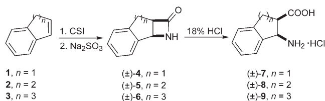
Scheme 1. Syntheses of compounds (±)-4 to (±)-9.
