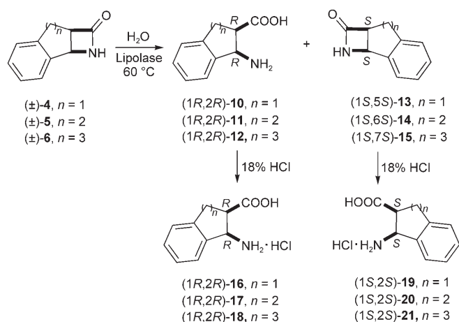
Scheme 2. Lipase-catalyzed enantioselective ring opening of compounds (±)-4 to (±)-6.
