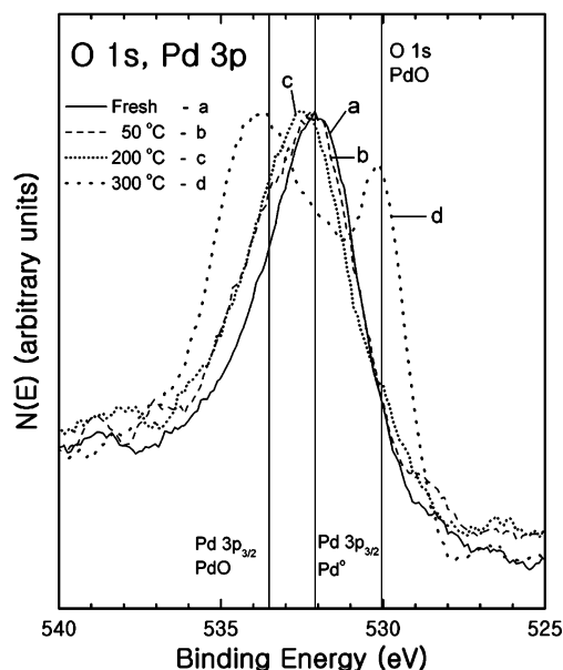
Figure 3. High-resolution XPS O 1s and Pd 3p spectra obtained from (a) fresh Pd metal powder and Pd metal powder after exposure to 0.5% O 2 for 60 min in the reactor at (b) 50, (c) 200, and (d) 300 °C. All Pd powders were prerduced with 3.5% H 2 in He at 100 °C for 60 min.
