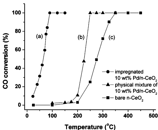
Figure 6. CO conversion as a function of temperature for (a) 10 wt % Pd/n-CeO 2 (impregnated), (b) a physical mixture of 0.010 g of Pd metal powder with sizes ranging from 0.25 to 0.55 \mu\text{m} and 0.090 g of nanocrystalline ceria, and (c) nanocrystalline ceria. The feed stream was 1.0% CO and 0.5% O 2 in He at a total flow rate of 45 cm 3 /min.
