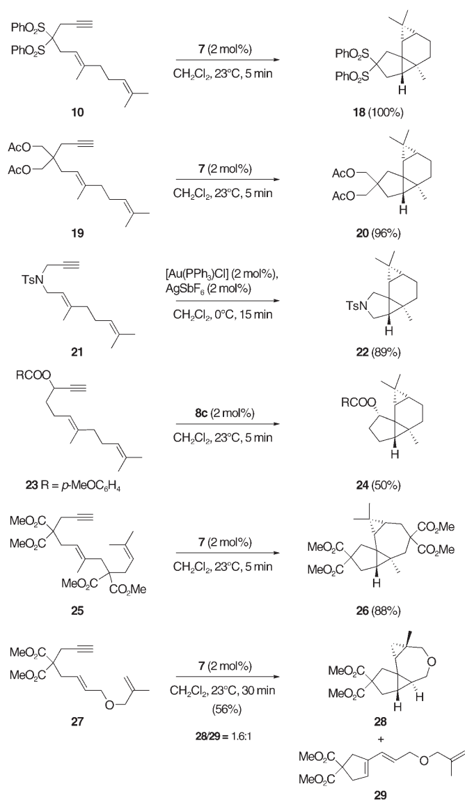
Scheme 6. Cyclization of dienes 10 , 19 , 21 , 23 , 25 , and 27 .
