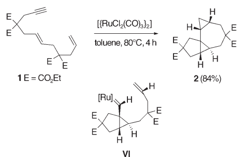
Scheme 2. Ru II -catalyzed biscyclopropanation of diyne 1 . [11]
