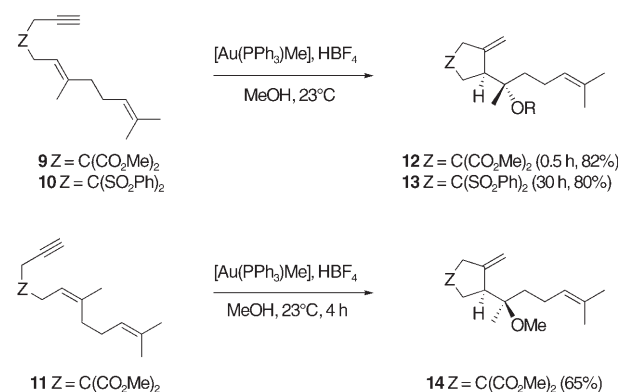
Scheme 5. Methoxycyclization of diynes 9–11 .
