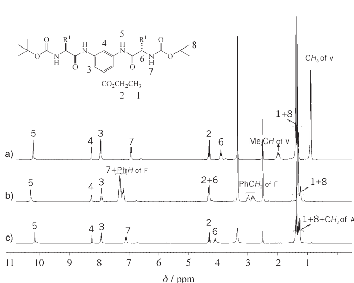
Figure 1. ^1\text{H} NMR (300 MHz) spectra of \text{G1}-(\text{aa}^1)_2\text{-CO}_2\text{Et} : a) \text{aa}^1\text{V} ( \text{R} = i\text{Pr} ), b) \text{aa}^1 = \text{F} ( \text{R} = \text{Bn} ), and c) \text{aa}^1\text{A} ( \text{R} = \text{Me} ) in [\text{D}_6]\text{DMSO} .
