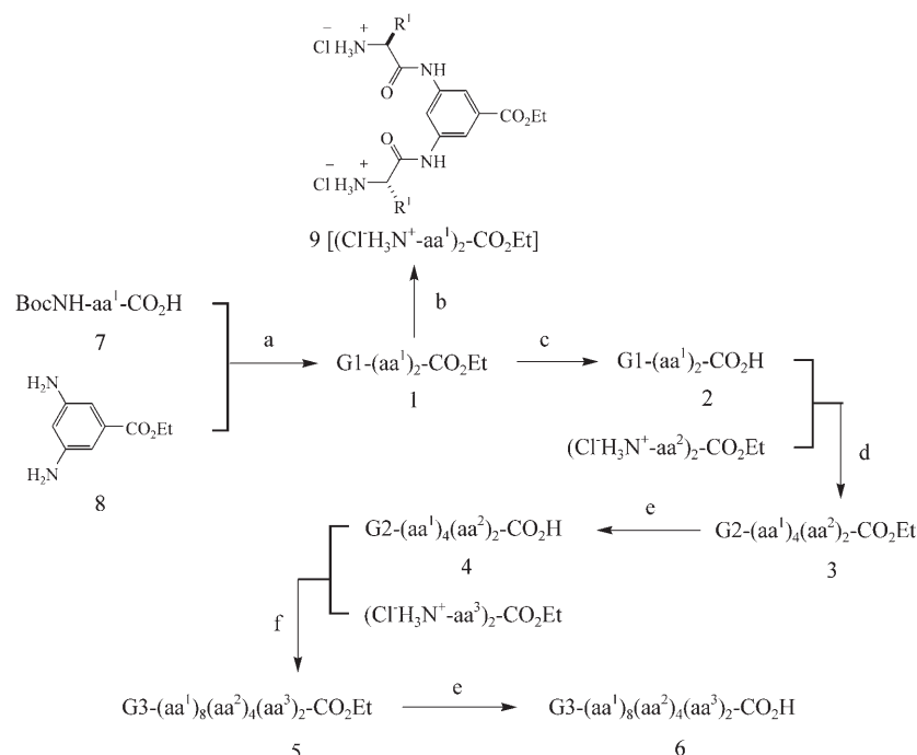
Scheme 1. Reagents and conditions: a) HOBt, DCC, THF, -10^{\circ}\text{C} to 25^{\circ}\text{C} , 11 h; b) HCl, EtOH, 25^{\circ}\text{C} , ~10 h; c) KOH (2.0 M), MeOH, \text{H}_2\text{O} , 25^{\circ}\text{C} , ~10 h; d) HOBt, DCC, 4-methylmorpholine, DMF, -10^{\circ}\text{C} to 25^{\circ}\text{C} , 50 h; e) KOH (2.0 M), MeOH, THF, \text{H}_2\text{O} , 25^{\circ}\text{C} , ~10 h; f) HOBt, EDCI, 4-methylmorpholine, DMF, -10^{\circ}\text{C} to 25^{\circ}\text{C} , 62 h.
