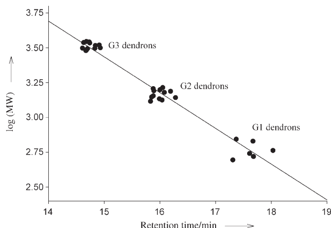
Figure 4. A plot of SEC retention time versus \log(MW) of the G1–G3 dendrons (solvent: 5% HOAc/DMF).
