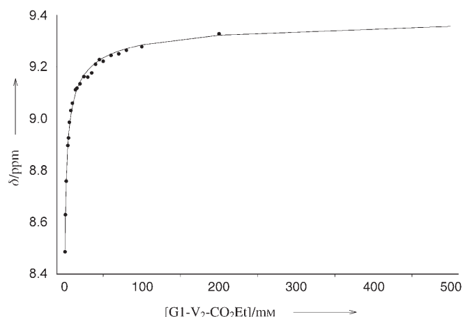
Figure 6. Concentration dependent 1 H NMR (300 MHz) chemical shift of the NHAr protons in G1-V 2 -CO 2 Et in CDCl 3 .
