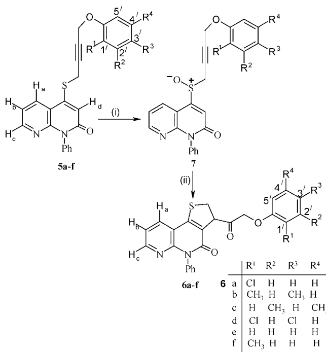
SCHEME 2 Reagents and reaction condition: (i) m -CPBA, dichloromethane, 0–5°C, 30 min (ii) Dichloromethane, reflux, 1 h.
