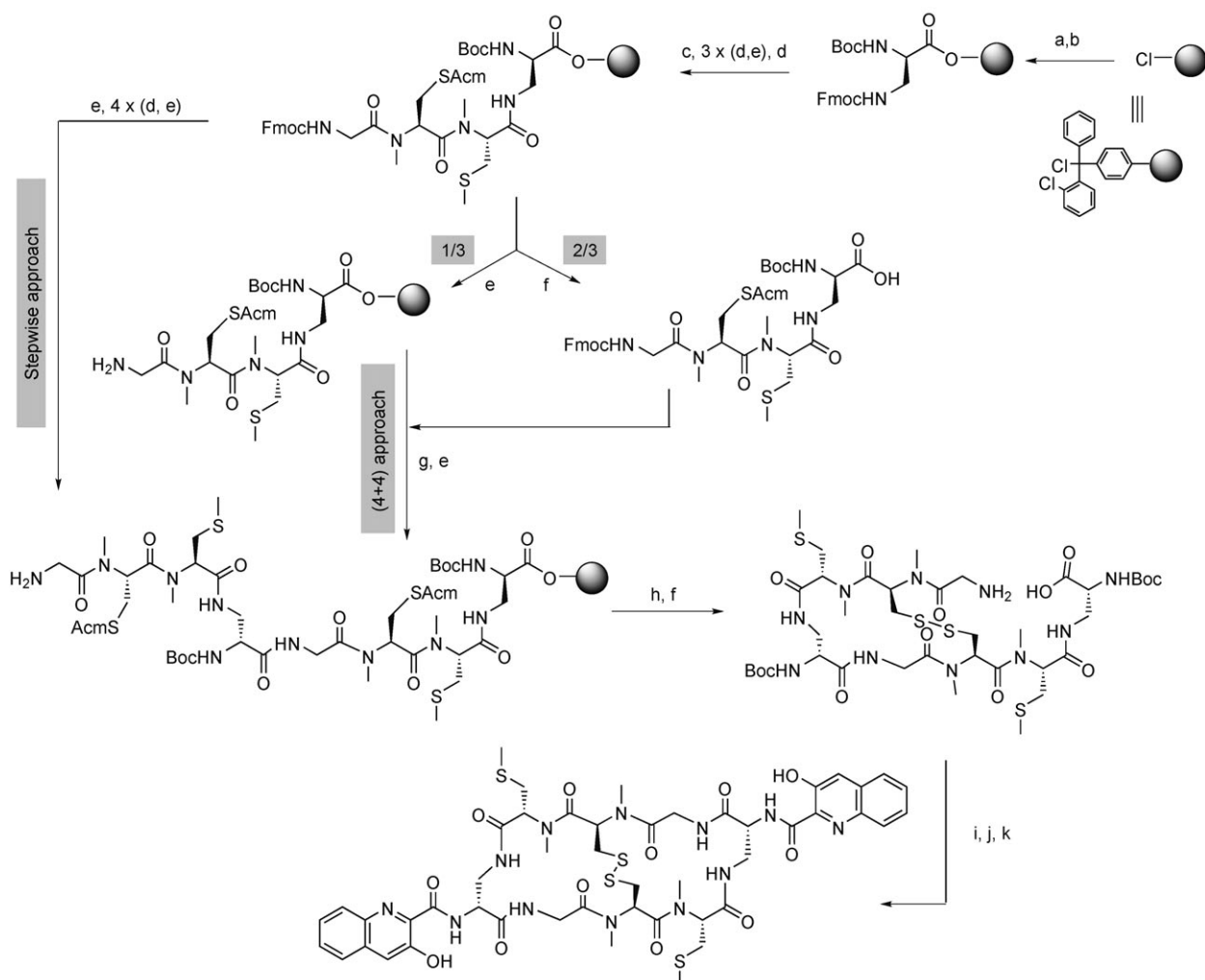
Scheme 2. Solid-phase strategy developed for the preparation of azathiocoraline by a (4+4) approach: a) Boc-D-Dap(Fmoc)-OH, DIEA, CH 2 Cl 2 ; b) MeOH; c) piperidine/DMF (1:4), piperidine/DBU/toluene/DMF (1:1:4:14); d) Fmoc-AA-OH/HATU/DIEA, DMF; e) piperidine/DMF (1:4); f) TFA/CH 2 Cl 2 (1:99); g) PyOAP/DIEA, CH 2 Cl 2 ; h) I 2 , DMF; i) EDC-HCl/HOAt/DIEA, CH 2 Cl 2 (1 mM); j) TFA/H 2 O (19:1); k) 3-Hydroxyquinaldic acid/EDC-HCl/HOSu/DIEA, CH 2 Cl 2 .
