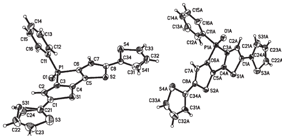
Figure 5. Molecular structure of 6f in the solid state (50% probability level). Selected bond lengths [Å]: P1–C3 1.806(2), P1–C6 1.800(2), P1–C11 1.804(2), C21–C1 1.494(4), C1–C2 1.378(3), C2–C3 1.408(3), C3–C4 1.387(3), C4–C5 1.448(3), C5–C6 1.392(3), C6–C7 1.408(3), C7–C8 1.382(3), C8–C34 1.455(3); P1A–C3A 1.804(2), P1A–C6A 1.811(3), P1A–C11A 1.797(2), C24A–C1A 1.460(3), C1A–C2A 1.371(3), C2A–C3A 1.409(3), C3A–C4A 1.382(3), C4A–C5A 1.448(3), C5A–C6A 1.382(3), C6A–C7A 1.406(3), C7A–C8A 1.374(3), C8A–C34A 1.468(3).
