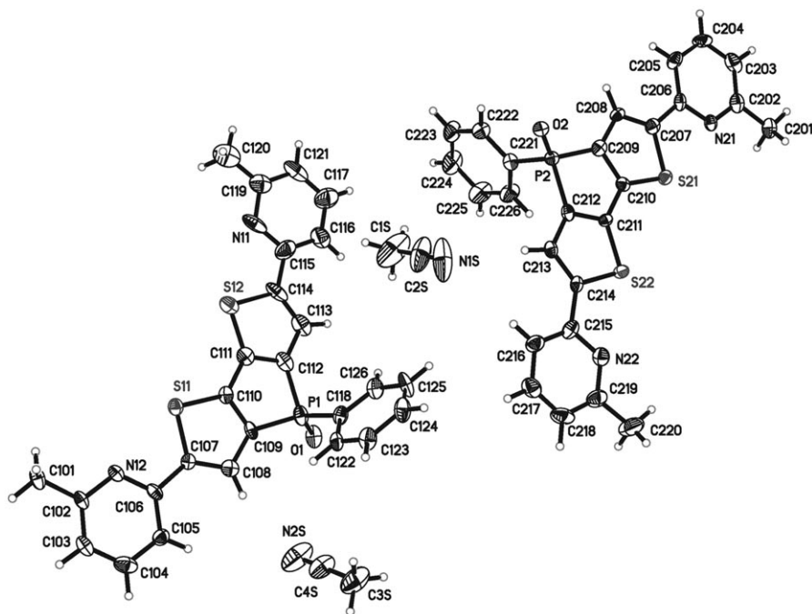
Figure 4. Molecular structure of 6e in the solid state (50% probability level). Selected bond lengths [Å]: P1–C118 1.790(6), P1–C109 1.799(6), P1–C112 1.798(7), C106–C107 1.461(8), C107–C108 1.371(8), C108–C109 1.396(8), C109–C110 1.372(8), C110–C111 1.466(8), C111–C112 1.376(8), C112–C113 1.378(8), C113–C114 1.348(9), C114–C115 1.443(10), P2–C221 1.816(5), P2–C209 1.798(6), P2–C212 1.819(6), C206–C207 1.451(8), C207–C208 1.370(8), C208–C209 1.435(8), C209–C210 1.390(8), C210–C211 1.454(8), C211–C212 1.373(8), C212–C213 1.397(8), C213–C214 1.370(8), C214–C215 1.471(8).
