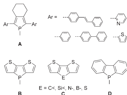
Figure 1. Phosphole- and dithieno-based materials.
