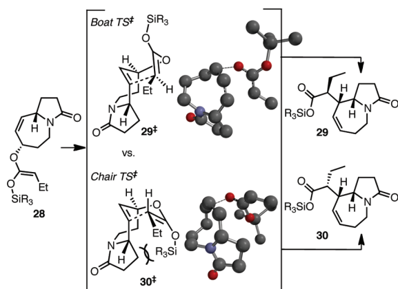
Scheme 8. Transition-State Analysis of the Ireland–Claisen Rearrangement
