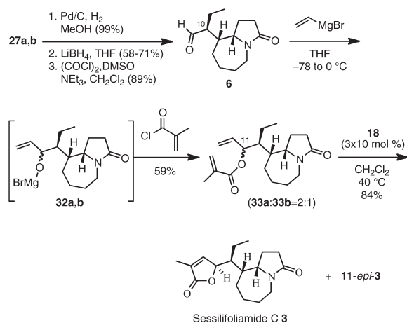
Scheme 10. Conversion of 27 to (–)-Sessilifoliamide C
