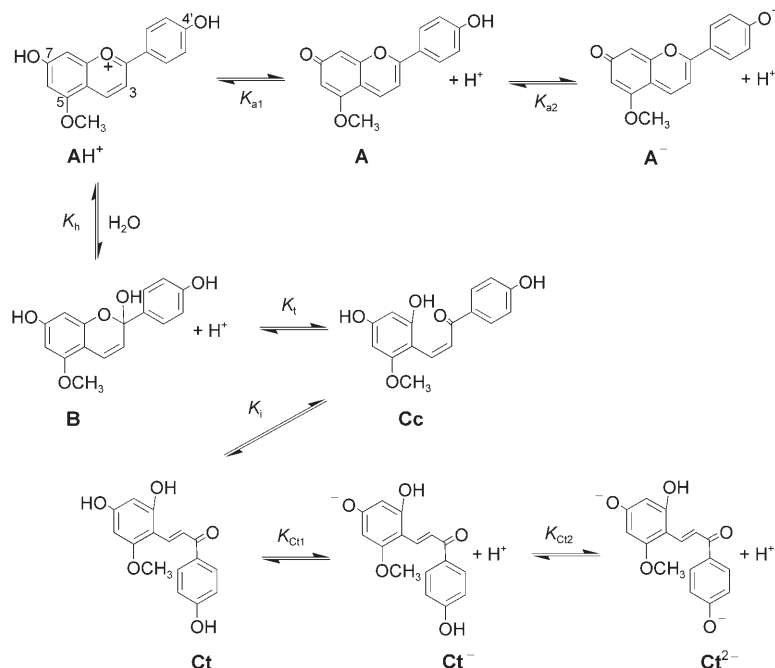
Scheme 1. Network of chemical reactions for dracoflavylum.
