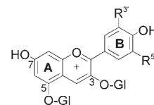
Scheme 2. In the basic chemical structure of anthocyanins, a hydroxyl group in positions 4' and 7 is present, and a sugar (Gl) in position 3 (monoglycosides) or positions 3 and 5 (diglycosides).
