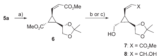
Scheme 4. Formation of cyclopropanecarboxylate 6 by oxidation of 5a and its reduction to alcohols 7 and 8 . a) \text{Py}^+-\text{O}^- , THF, \text{H}_2\text{O} , 25^\circ\text{C} , 94%; b) for 7 : \text{LiAlH}_4 , THF, -50^\circ\text{C} , 87%; c) for 8 : \text{LiAlH}_4 , THF, -50 to 25^\circ\text{C} , 94%.
