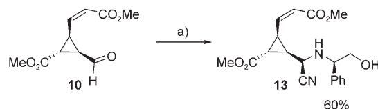
Scheme 6. Strecker aminocyanation on aldehyde 10 . a) i) ( R )-(-)-2-phenylglycinol, \text{MeOH} , 25^\circ\text{C} , ii) \text{TMS-CN} , -10^\circ\text{C} . \text{TMS-CN} = trimethylsilyl cyanide.
