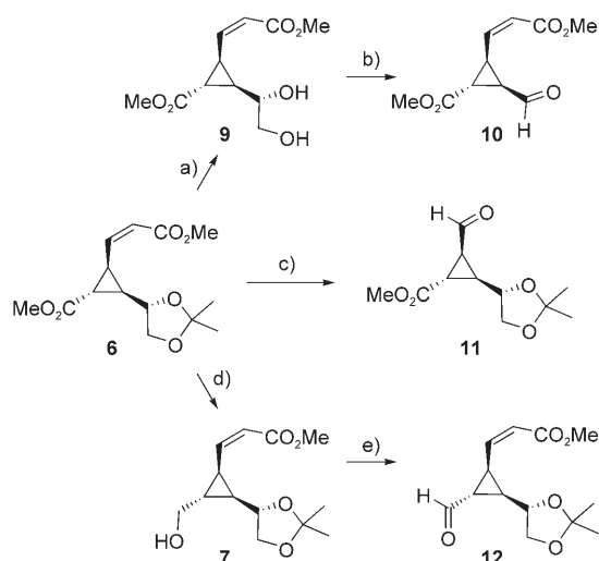
Scheme 5. Synthesis of the enantiopure cyclopropanecarbaldehydes 10 , 11 and 12 . a) \text{HCl} (6N), THF, 25^\circ\text{C} , 96%; b) \text{NaIO}_4 , \text{CH}_2\text{Cl}_2 , \text{H}_2\text{O} , pH 7.2, 25^\circ\text{C} , 89%; c) i) \text{O}_3 , \text{CH}_2\text{Cl}_2 , \text{MeOH} , -78^\circ\text{C} , ii) \text{SMe}_2 , -78 to 25^\circ\text{C} , 93%; d) \text{LiAlH}_4 , THF, -50^\circ\text{C} , 87%; e) \text{PCC} , \text{CH}_2\text{Cl}_2 , 25^\circ\text{C} , 91%. \text{PCC} = pyridinium chlorochromate.
