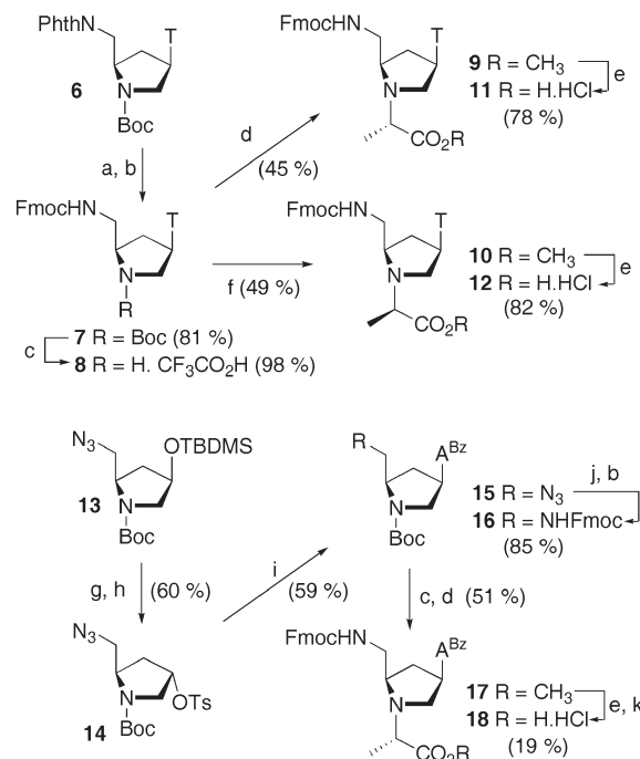
Scheme 1 Synthesis of MePOM Fmoc-monomers. (a) 40% aq. MeNH 2 , 50 ^{\circ}\text{C} , 2 h; (b) Fmoc-Cl, 10% (w/v) aq. Na 2 CO 3 , dioxane, 0 ^{\circ}\text{C} \rightarrow rt, 18 h; (c) 20% CF 3 COOH in CH 2 Cl 2 , rt, 4 h; (d) (2R)-methyl 2-bromopropionate, 10 DIPEA, DMF, 0 ^{\circ}\text{C} \rightarrow rt, 18 h; (e) 2 M HCl aq., reflux 18 h; (f) (2S)-methyl 2-bromopropionate, 10 DIPEA, DMF, 0 ^{\circ}\text{C} \rightarrow rt, 18 h; (g) TBAF, THF, rt 18 h; (h) CH 3 OTs, PPh 3 , DIAD, THF, -10 ^{\circ}\text{C} \rightarrow rt, 18 h; (i) N 6 -benzoyladenine, K 2 CO 3 , 18-crown-6, DMF, 80 ^{\circ}\text{C} , 18 h; (j) sat. H 2 S in 60% aq. pyridine, 18 h; (k) benzyl-Cl, anhydrous pyridine, reflux, 2 h. T = thymine-1-yl, A Bz = N 6 -benzoyladenine-9-yl, Phth = phthaloyl.
