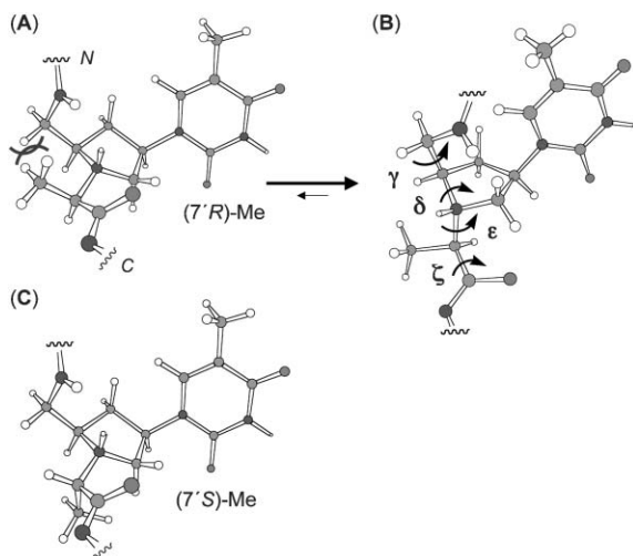
Fig. 2 Idealised helical conformations of MePOMs. (A) (7' R )-MePOM in an A-type conformation with pyrrolidine ring in the N1'-endo pucker which is described by the pseudorotation phase angle ( P ) of 45° and \delta = 75^\circ . 5b (B) (7' R )-MePOM in a B-type, N1'-exo conformation ( P = 195°, \delta = 155^\circ ). (C) (7' S )-MePOM in an A-type, N1'-endo conformation ( P = 45°, \delta = 75^\circ ) conformation. In accord with X-ray crystallographic and other data 5b the \gamma and \epsilon torsion angles are set at ca. 60° and 180° respectively.
