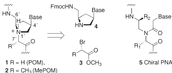
Fig. 1 Structure of POM, (7′ S )-MePOM and chiral Peptide Nucleic Acids (PNAs). Chiral αPNAs have improved DNA/RNA recognition properties (e.g. 5 , R 1 = (CH 2 ) 4 NH 2 ) 7 and improved transport and distribution within cells ( 5 , R 1 = carbohydrates or (CH 2 ) 3 NHC(=NH 2 )NH 2 ) 8 . PNAs substituted with a fluorophore at the γ-position ( 5 , R 2 = fluorene) can also be used as molecular beacons. 9a Base = A, T, C or G.
