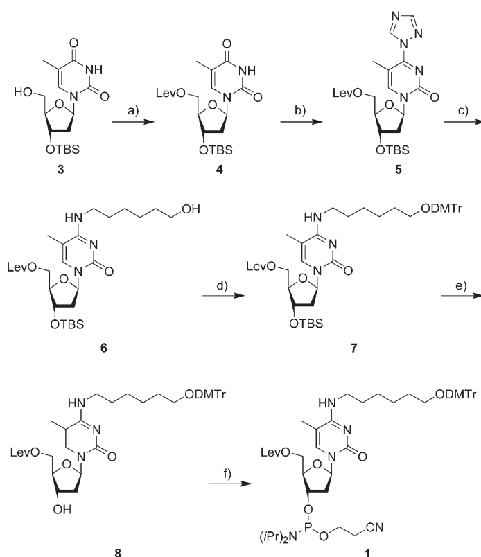
Scheme 2. Synthesis of phosphoramidite 1 : a) 2-chloro-1-methylpyridinium iodide, DABCO, levulinic acid, CH 3 CN/dioxane, 90%; b) 1,2,4-triazole, NEt 3 , POCl 3 , CH 3 CN, 100%; c) 6-aminohexanol, CH 3 CN, 88%; d) DMTr-Cl, DMAP, pyridine, 88%; e) AcOH/TBAF, THF, 90%; f) DIPEA, O -(2-cyanoethyl)- N,N' -diisopropylchlorophosphoramidite, CH 2 Cl 2 , 97%. (TBS = tert -butyldimethylsilyl)
