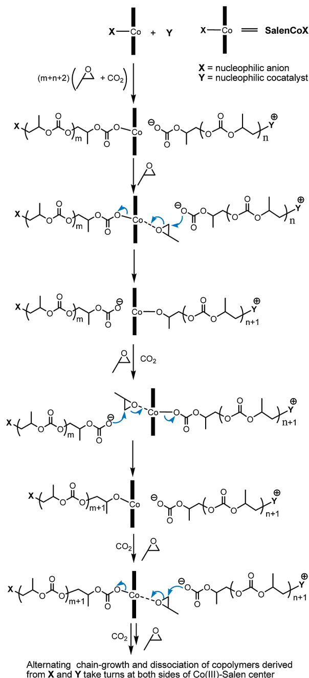
Scheme 3. Mechanistic Understanding of Binary Catalyst Systems Based on SalenCo(III) for CO 2 /PO Copolymerization
