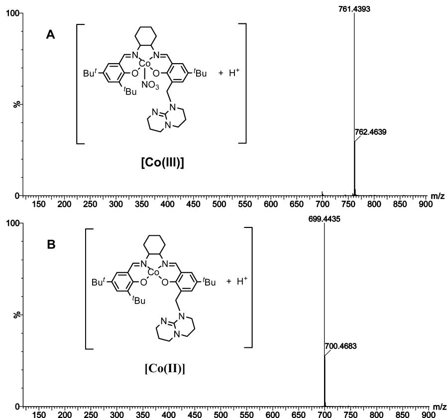
Figure 4. ESI-Q-TOF mass spectra of (A) the complex 5 in \text{CH}_2\text{Cl}_2 , and (B) the reaction mixture of PO and \text{CO}_2 catalyzed by the complex 5 ( \text{5/PO} = 1/10\,000 , molar ratio) at 25^\circ\text{C} and 1.5 MPa.
