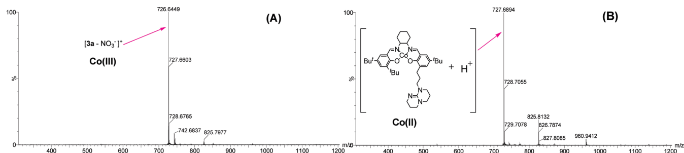
Figure 5. Detailed ESI-Q-TOF mass spectra of the reaction mixture of CHO and CO 2 catalyzed by 3a ( 3a /CHO = 1/5000, molar ratio) at 25 °C with various time points: (A) 5 min, and (B) 2 h (diluted with CH 2 Cl 2 ).
