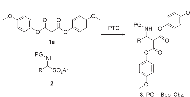
Scheme 1. Catalytic asymmetric Mannich reaction with malonate 1a . PTC: phase-transfer catalysis.
