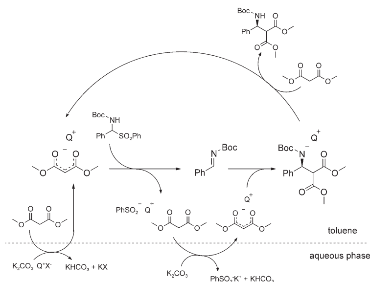
Scheme 3. Proposed reaction pathway. ( Q^+X^- = 4e ).
