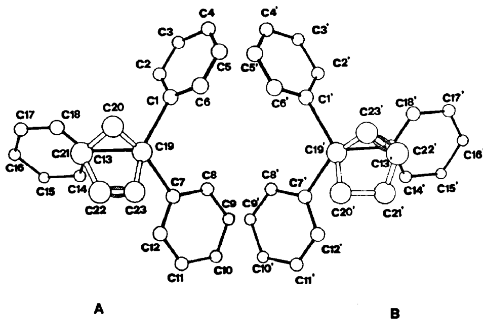
Fig. 1. Structure of cyclopent-2-enyltriphenyltin with atom numbering. The two molecules A and B forming the asymmetric unit are viewed down the \text{C}(19)\text{--Sn}(\text{C}(19)'\text{--Sn}') axis and suitably oriented in order to show the pseudo-mirror symmetry between the triphenyltin groups. The configurations of the \text{C}_5 rings of A and B are the same.
