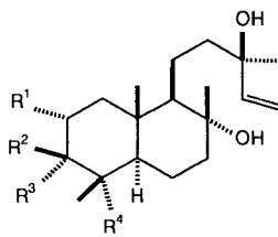
4 R 1 = R 2 = H, R 3 = OH, R 4 = CH 3
