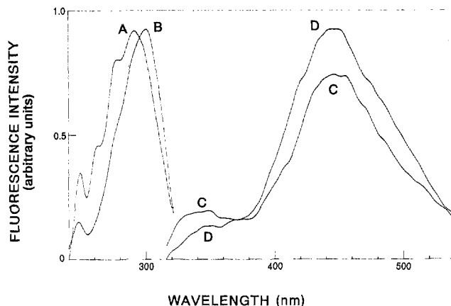
Figure 1. Luminescence dependence on excitation wavelength for ester 1 ( 10^{-6}\text{ M} ) in \text{CHF}_3 at 28^\circ\text{C} and 102.0 bar. Curve A: excitation spectrum monitored at 350 nm; maximum 291 nm. Curve B: excitation spectrum monitored at 434 nm (intensity divided by a factor of five); maximum 300 nm. Curve C: emission spectrum for excitation at 282 nm; maxima 350 and 444 nm. Curve D: emission spectrum for excitation at 298 nm; maximum 446 nm. Curves C and D are corrected for relative absorbance efficiency. Data collected in ratio mode.
