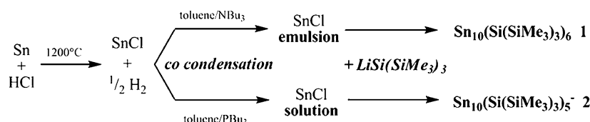
Scheme 1. Schematic Presentation of the Synthesis of Metalloid Sn-Clusters Applying Various Sn(I) Halide Precursors (Emulsion or Solution) Depending on the Donor Applied During the Cocondensation Reaction
