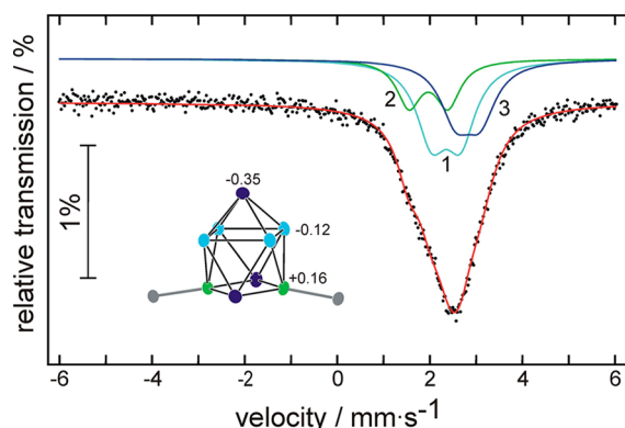
Figure 3. Experimental and simulated ^{119}\text{Sn} Mössbauer spectrum of \{\text{Sn}_9[\text{Si}(\text{SiMe}_3)_3]_2\}\{\text{Li}(\text{TMEDA})_2\}_2 at 78 K. The subspectra of the tin species 1, 2, and 3 are drawn in blue, green, and violet, similar to the tin cluster. The calculated charges of the three sets of tin atoms are indicated.
