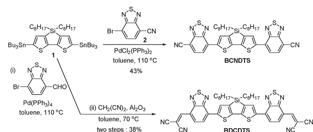
Scheme 1. Synthesis of BCNDTS and BDCDTS
