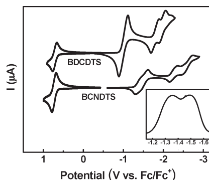
Figure 1. Cyclic voltammograms of BCNDTS and BDCDTS . All potentials were recorded versus ferrocene/ferrocenium ( \text{Fc}/\text{Fc}^+ ) as an external reference. Inset: the selected reduction region of the differential pulse voltammogram of BCNDTS . Scan rate: 100 mV/s.
