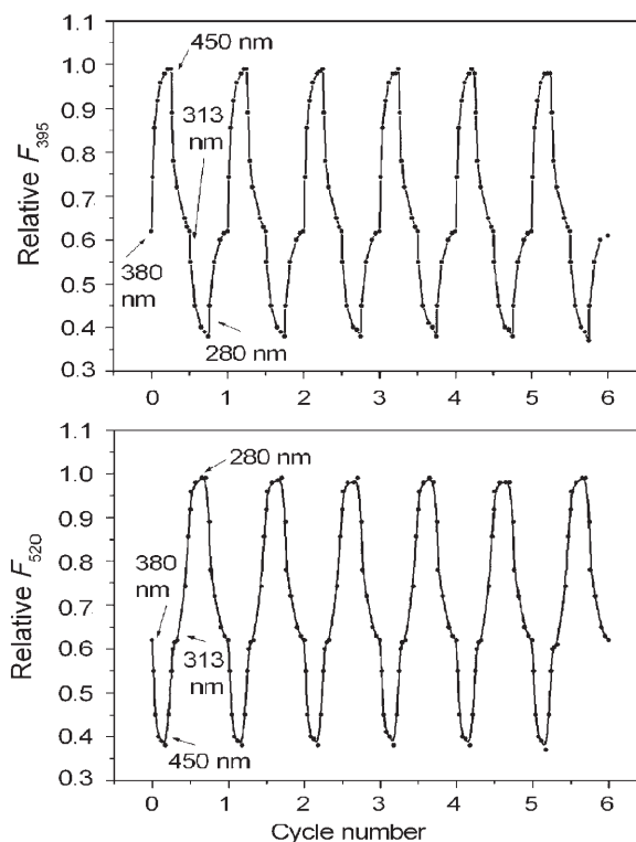
Figure 7. Changes in the fluorescence spectra of the “S” stopper (top, \lambda_{\text{ex}} = 336 nm, emission at \lambda_{\text{max}} = 395 nm), and the “N” stopper (below, \lambda_{\text{ex}} = 438 nm, emission at \lambda_{\text{max}} = 520 nm) of a NNAS-2CD solution ( 1.0 \times 10^{-5} M in DMF) along with changes in irradiation cycle and light sources. In one cycle, 380 nm and 450 nm irradiation was first used to isomerize and recover the azobenzene unit, then 313 nm and 280 nm irradiation was used to isomerize and recover the stilbene unit. The photochemical processes are highly reproducible over more than six cycles.
