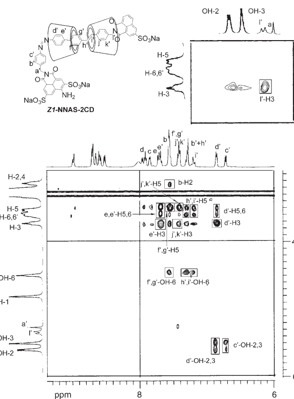
Figure 2. The two-dimensional ^1\text{H} ROESY NMR spectrum (500 MHz in [\text{D}_6]\text{DMSO} at 298 K; mixing time 300 ms) of NNAS-2CD after irradiation at 380 nm for 2 h.
