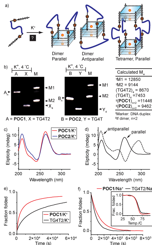
Figure 2. (a) Alternative folded structures of self-assembled POCs. (b) PAGE images showing POCs are forming dimeric complexes according to their electromobility shifts. (c and d) CD spectra of the POC complexes and known parallel and antiparallel G-quadruplexes. (e) Kinetics of G-quadruplex formation of POC1 and TG4T2 . (f) Dissociation kinetics of the complexes at their T_{1/2} ; inset shows their melting profile.
