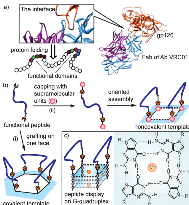
Figure 1. (a) An example of antigen–antibody interactions: gp120 (HIV envelope protein; orange)–VRC01 (antibody for gp120; V H in blue, V L in magenta), pdb 3NGB. (b) Covalent (i) and noncovalent (ii) strategies for mimicking multiloop surfaces. (c) Display of two constrained peptides on one face (5′) of G-quadruplex.
