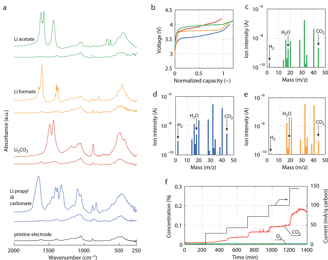
Figure 5. Composite electrodes (Super P/ \alpha -MnO 2 /Kynar) that contain the discharge products individually were subjected to charging in 1 M LiPF 6 in PC under O 2 . (a) FTIR spectra of the as-prepared electrodes and the charged electrodes for each of the compounds, together with the spectrum of a pristine electrode. (b) The corresponding charging curves at 70 mA/g (based on mass of carbon). Since the theoretical capacities of the different compounds vary, to aid comparison the capacities are all normalized to unity (theoretical capacities: Li propyl dicarbonate 1000 mA h/g, 2 e - /mol; Li 2 CO 3 1500 mA h/g, 2 e - /mol; CH 3 CO 2 Li 750 mA h/g, 1 e - /mol; HCO 2 Li 750 mA h/g, 1 e - /mol). (c–e) MS gas analysis at the end of charging under O 2 of CH 3 CO 2 Li (c), C 3 H 6 (OCO 2 Li) 2 (d), and HCO 2 Li (e). Note that unmarked peaks arise from fragments of CO 2 , H 2 O, O 2 , and Ar. (f) Gas evolution measured by DEMS on oxidation of a composite electrode containing Li 2 CO 3 in response to a stepwise increased current under Ar.
