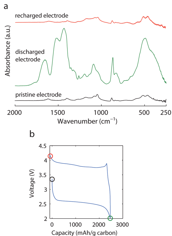
Figure 4. (a) FTIR spectra of a pristine electrode (Super P/ \alpha - \text{MnO}_2 /Kynar) and after the first discharge, then charge in 1 M \text{LiPF}_6 in PC under \text{O}_2 . (b) Variation of voltage as cell is discharged then charged.
