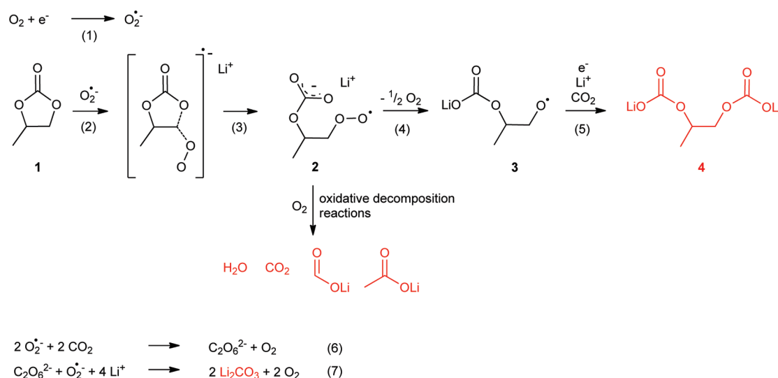
Scheme 1. Proposed Reaction Scheme on Discharge To Explain Formation of the Compounds: Li Propyl Dicarbonate, Li Formate, Li Acetate, \text{Li}_2\text{CO}_3 , \text{CO}_2 , and \text{H}_2\text{O} a
