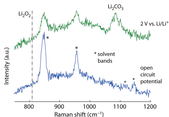
Figure 3. SERS on an Au electrode in 1 M \text{LiPF}_6/\text{PC} under \text{O}_2 at open circuit potential and after discharge to 2 V. The dashed line marks the position where \text{Li}_2\text{O}_2 , if present, would occur.
