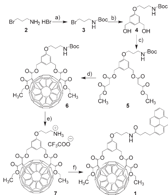
Scheme 1. a) (BOC) 2 O, TEA, CH 2 Cl 2 ; b) 3,5-bis(hydroxymethyl)phenol, K 2 CO 3 , acetone; c) ethyl malonyl chloride, TEA, CH 2 Cl 2 ; d) C 60 , DBU, I 2 , toluene; e) CF 3 COOH, CH 2 Cl 2 ; f) 1-pyrene butyric acid, HOBT, EDCI, 4-methylmorpholine (for abbreviations, see text).
