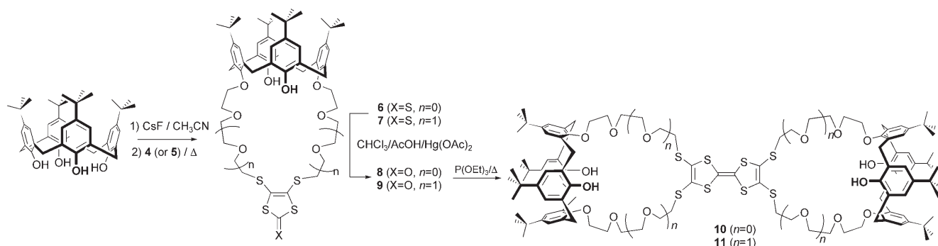
Scheme 2. Synthesis of the calix–crown–TTF assemblies 10 and 11 .
