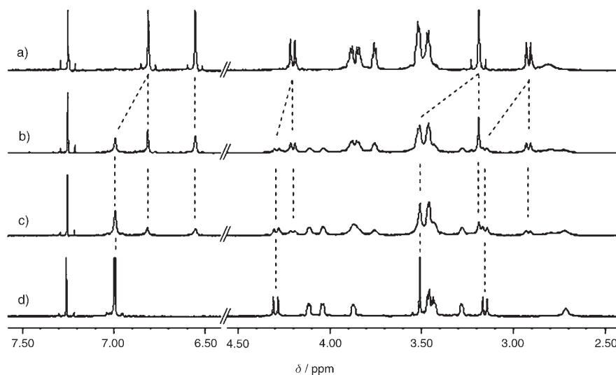
Figure 2. ^1\text{H} NMR spectra of 15 ( \text{CDCl}_3/\text{CD}_3\text{CN} ) in the presence of \text{NaClO}_4 : a) [\text{Na}^+]/[\text{15}] = 0.0 ; b) [\text{Na}^+]/[\text{15}] = 0.5 ; c) [\text{Na}^+]/[\text{15}] = 1.0 ; d) [\text{Na}^+]/[\text{15}] = 2.0 .
