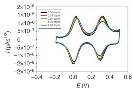
Figure 5. Deconvoluted CV of 13 (0.26 mM) in CH 3 CN/CH 2 Cl 2 /TBAPF 6 (0.10M) in the presence of increasing amounts of NaClO 4 ; Pt electrode ( \varnothing 1.6 mm, \nu = 100 mV s -1 , versus Fc +/0 /Fc).
