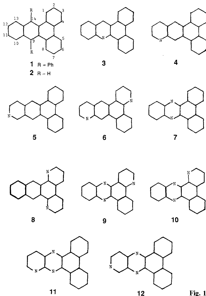
Fig. 1. Isoskeletal analogs of dibenzo[a,c]anthracene
