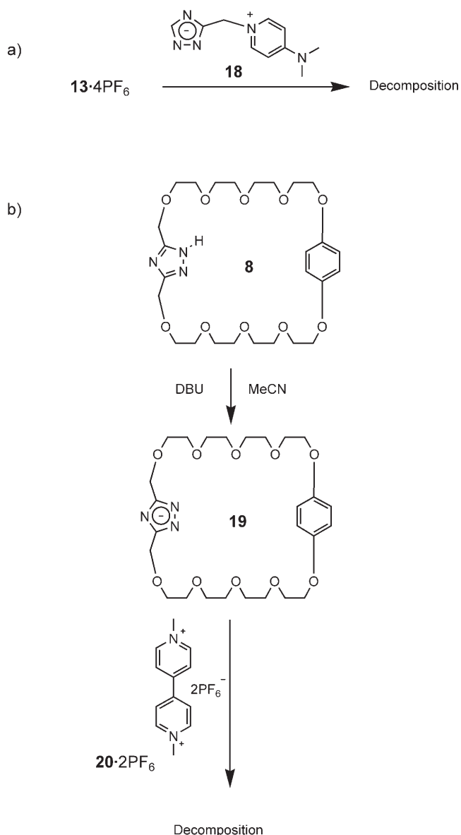
Scheme 4. Effect of triazolate ions on different 4,4'-bipyridinium derivatives.
