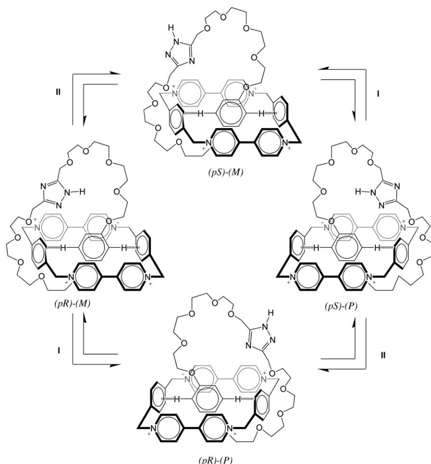
Figure 1. Processes I and II for interconverting diastereoisomers and inverting enantiomers of [2]catenane 13^{4+} . Process I corresponds to a change in helical chirality, while process II represents alteration of planar chirality. The descriptors of absolute stereochemistry are defined in Figure 2.
