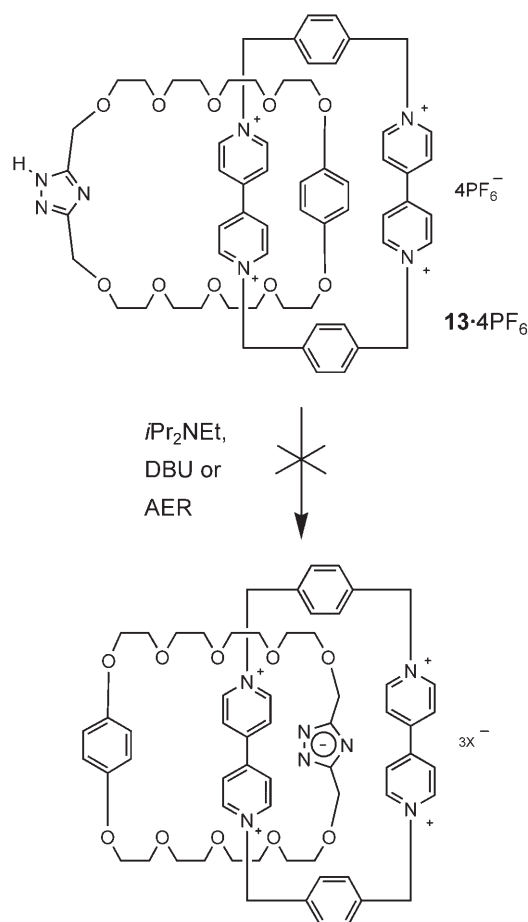
Scheme 3. Treatment of [2]catenane 13 ·4PF 6 with different bases.
