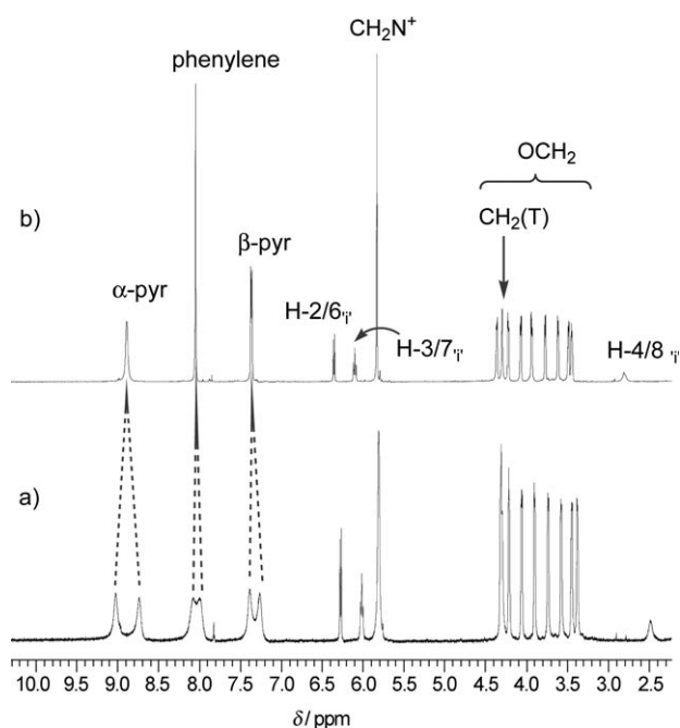
Figure 8. 1 H NMR spectrum of [2]catenane 14·4PF 6 in CD 3 CN at a) 298 K; b) 363 K.
