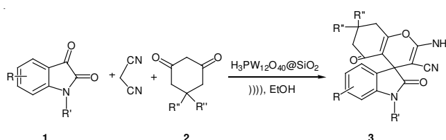
Scheme-I: Reaction of isatins, 1,3-cyclohexadione and malononitrile in the presence of silica supported of tungstophosphoric acid under ultrasound irradiation
