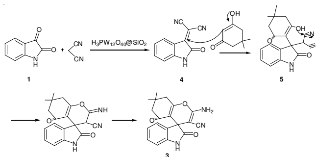
Scheme-II: Proposed mechanism for synthesis of spirooxindoles
