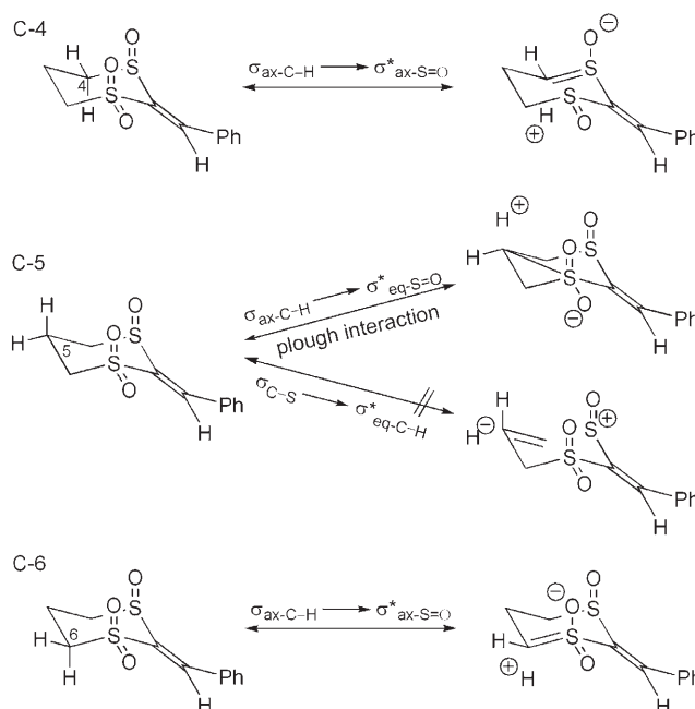
Figure 6. Explanation of Perlin effects dithiane-derived sulfoxide-sulfone 10 .
